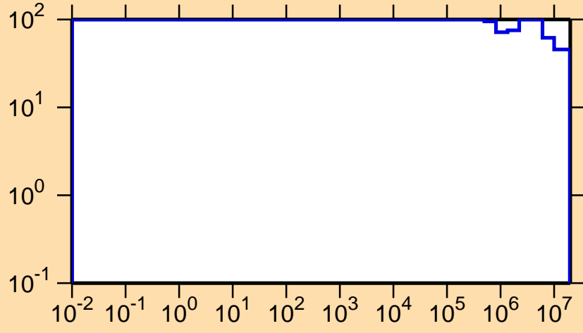
\Delta\sigma/\sigma vs. E for ^{240}\text{Bk}(n,p)
