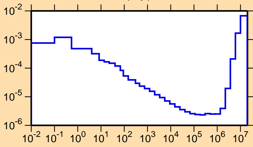
\sigma vs. E for ^{240}\text{Bk}(n,p)
