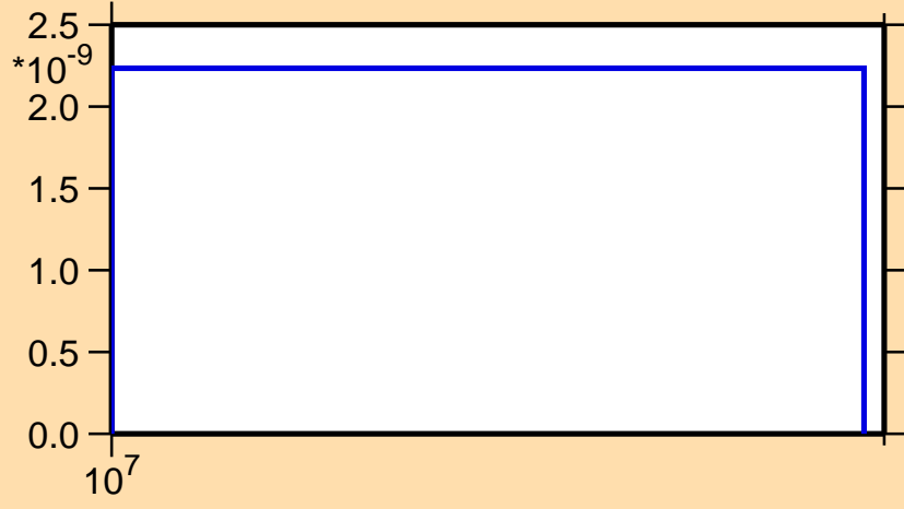
\sigma vs. E for ^{240}\text{Bk}(n,nt)
