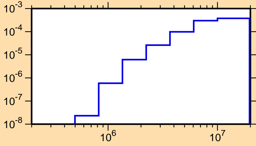
\sigma vs. E for ^{240}\text{Bk}(n,n_3)
