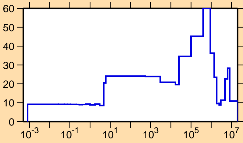
\Delta\sigma/\sigma vs. E for ^{240}\text{Bk}(n,el.)
