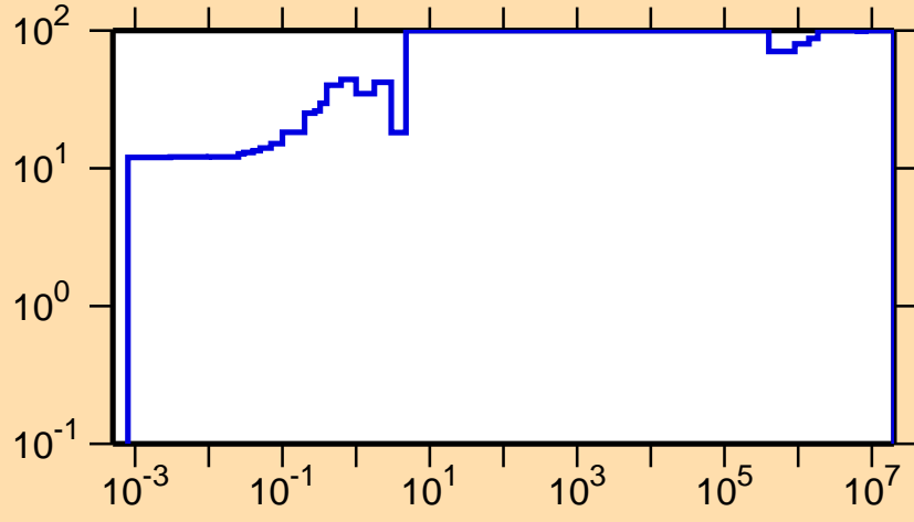
\Delta\sigma/\sigma vs. E for ^{240}\text{Bk}(n,\gamma)
