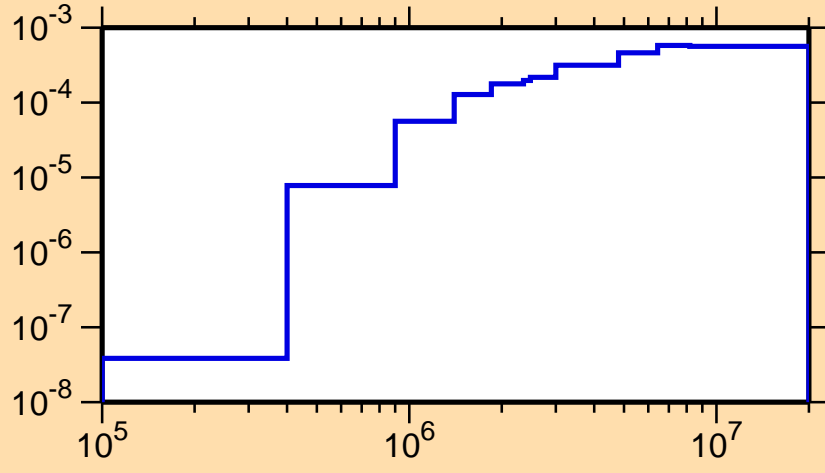
\sigma vs. E for ^{240}\text{Bk}(n,n_4)
