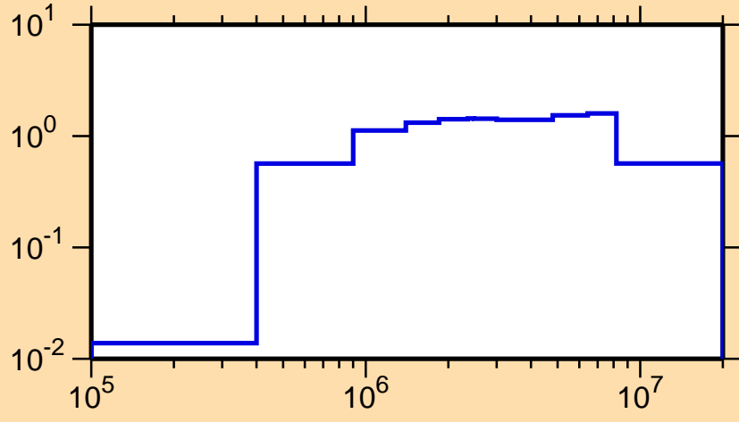
\sigma vs. E for ^{240}\text{Bk}(n,n\text{cont.})
