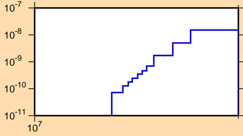
\sigma vs. E for ^{241}\text{Bk}(\text{mt } 45)
