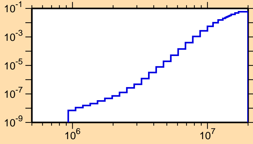
\sigma vs. E for ^{241}\text{Bk}(n,p)
