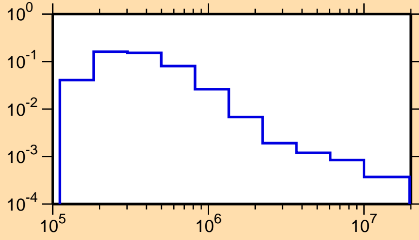
\sigma vs. E for ^{241}\text{Bk}(n,n_3)
