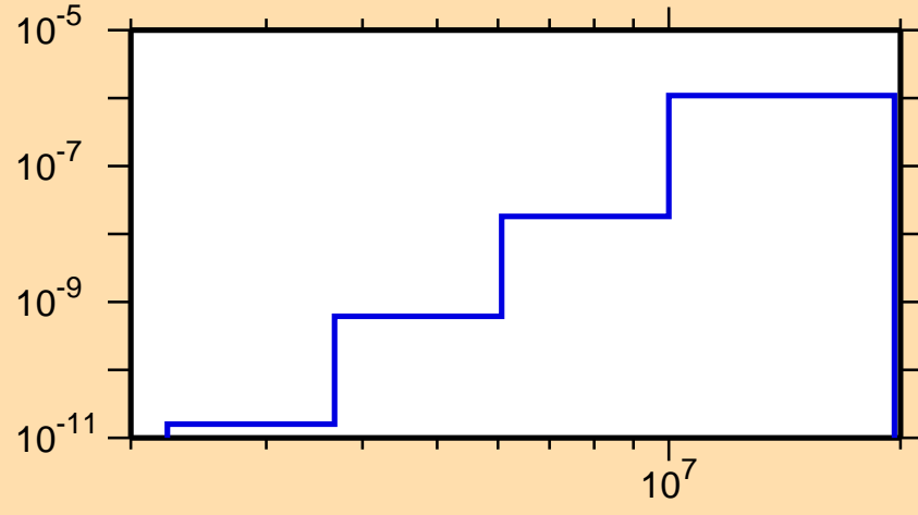
\sigma vs. E for ^{241}\text{Bk}(n,p\alpha)
