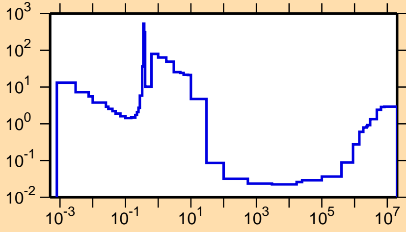
\sigma vs. E for ^{241}\text{Bk}(n,f)
