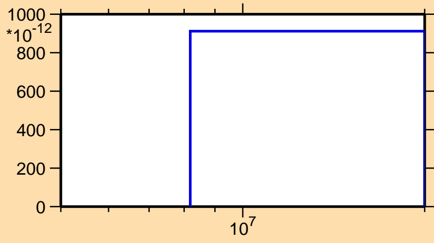
\sigma vs. E for ^{241}\text{Bk}(\text{mt117})
