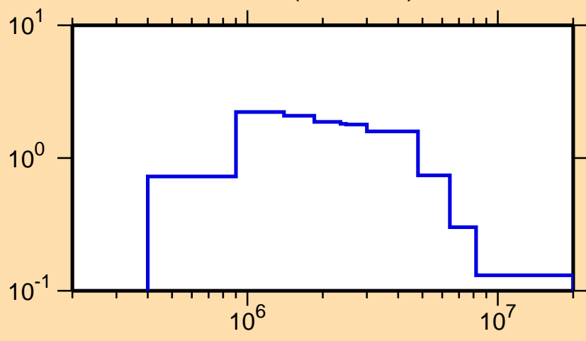
\sigma vs. E for ^{241}\text{Bk}(n,n\text{cont.})
