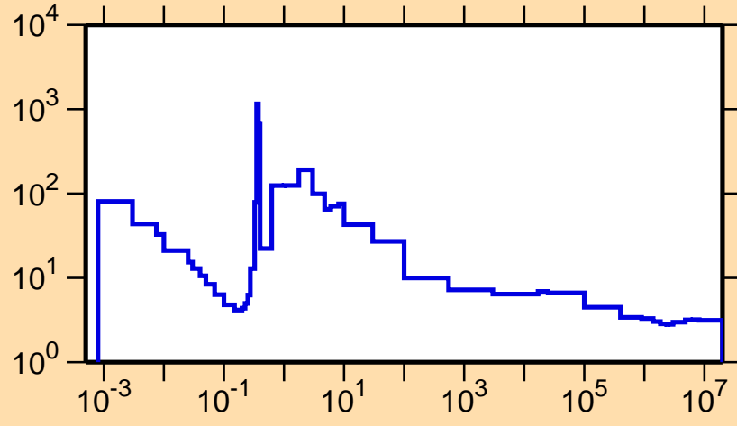
\sigma vs. E for ^{241}\text{Bk}(n,\text{nonel.})
