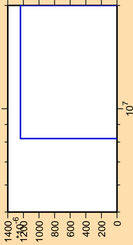
\Delta\sigma/\sigma vs. E for ^{241}\text{Bk}(n,3n\alpha)
