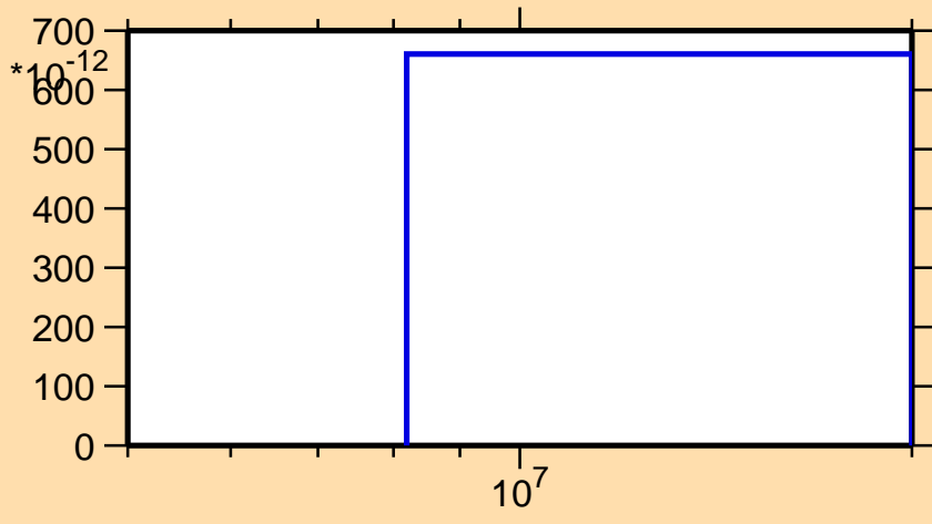
\sigma vs. E for ^{241}\text{Bk} (mt 45)
