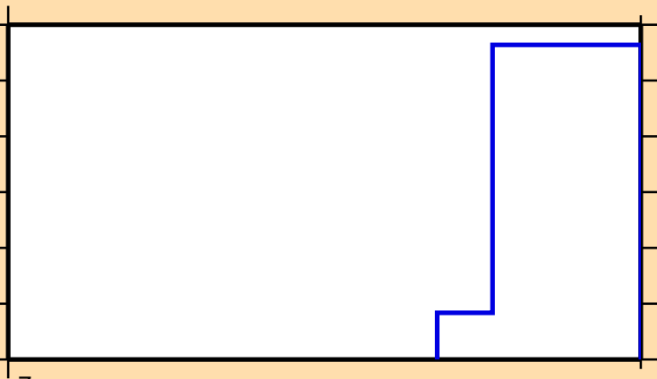
\sigma vs. E for ^{242}\text{Bk}(\text{mt117})
