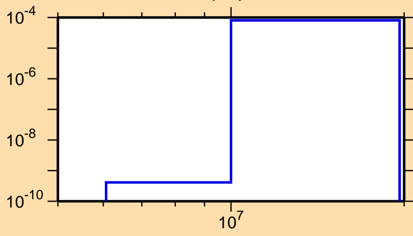
\sigma vs. E for ^{242}\text{Bk}(n,t)
