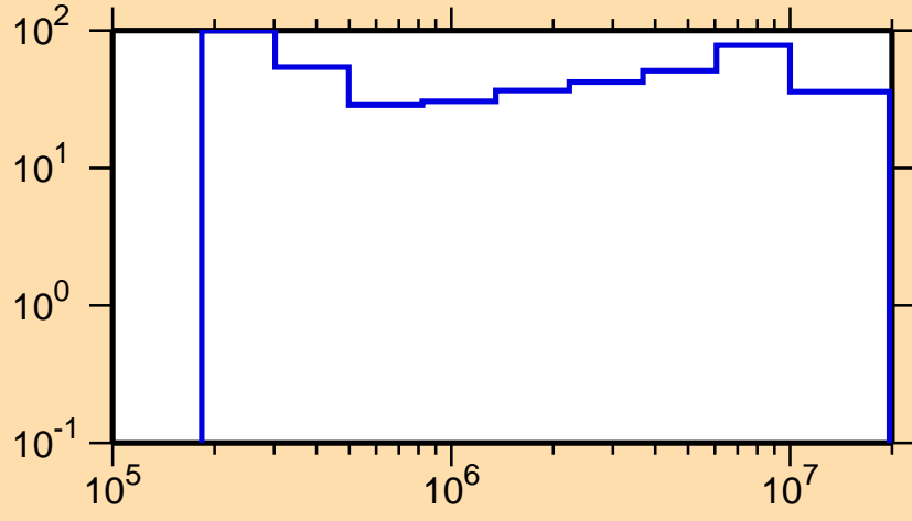
\Delta\sigma/\sigma vs. E for ^{242}\text{Bk}(n,n\text{cont.})
