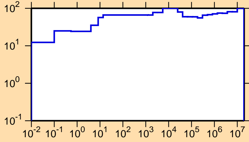
\Delta\sigma/\sigma vs. E for ^{242}\text{Bk}(n,\gamma)
