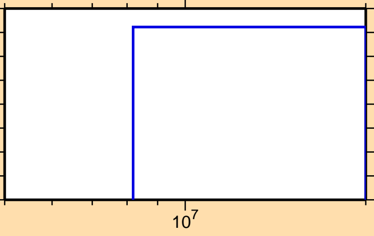
\sigma vs. E for ^{242}\text{Bk} (mt 34)
