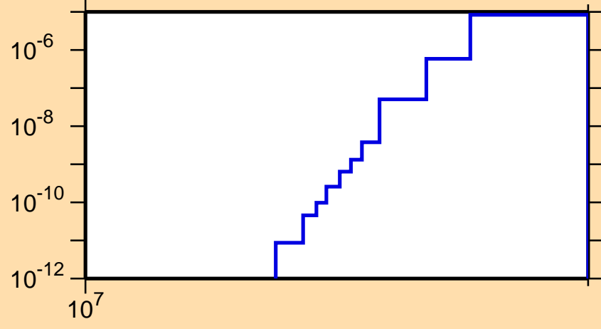
\sigma vs. E for ^{243}\text{Bk}(n,nd)
