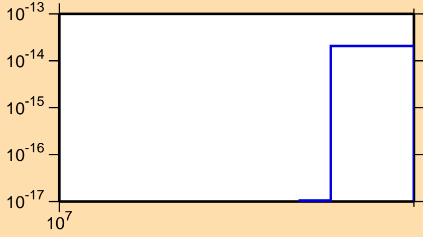
\sigma vs. E for ^{243}\text{Bk} (mt 11)
