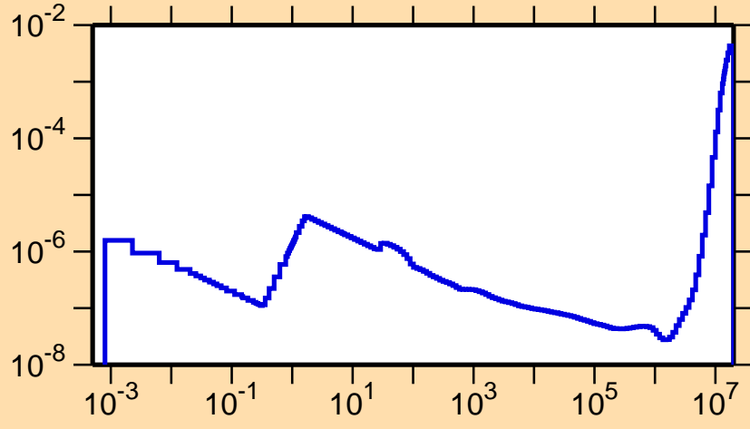
\sigma vs. E for ^{243}\text{Bk}(n,\alpha)
