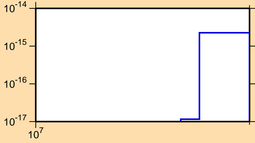
\sigma vs. E for ^{243}\text{Bk} (mt 34)
