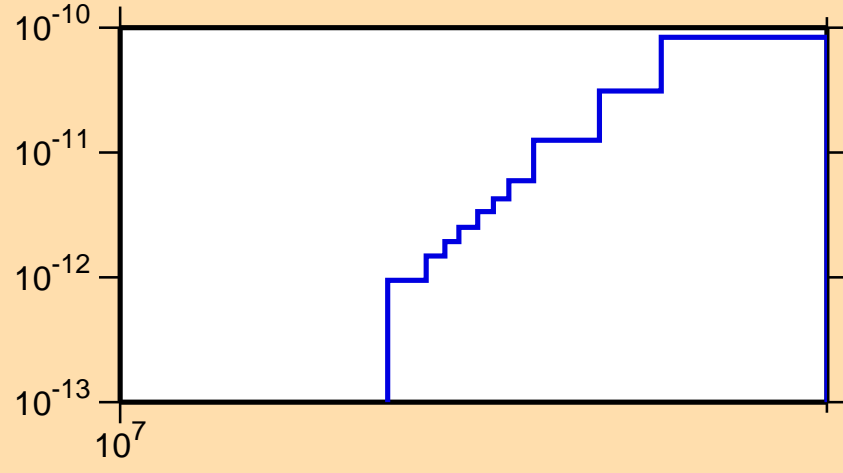
\sigma vs. E for ^{243}\text{Bk}(n,p\alpha)
