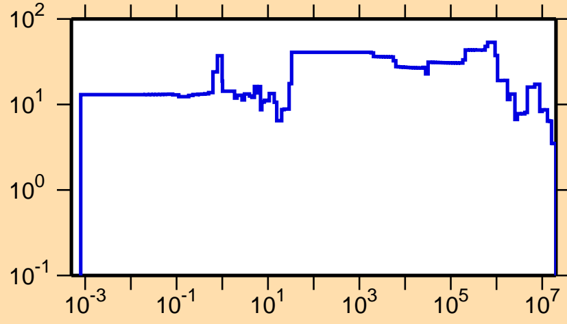
\Delta\sigma/\sigma vs. E for ^{243}\text{Bk}(n,el.)
