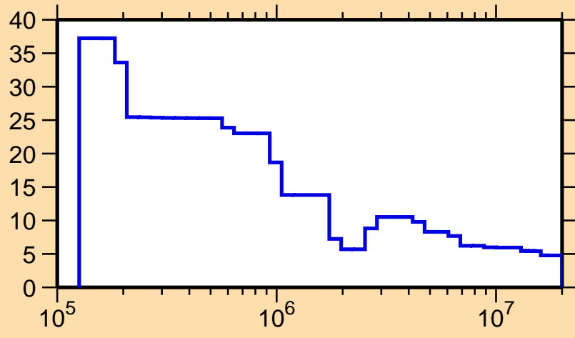
\Delta\sigma/\sigma vs. E for ^{244}\text{Bk}(n,\text{nonel.})
