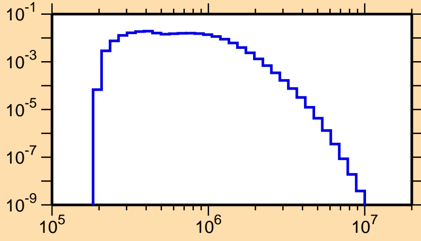
\sigma vs. E for ^{244}\text{Bk}(n,n_4)
