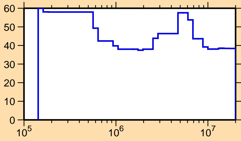
\Delta\sigma/\sigma vs. E for ^{244}\text{Bk}(n,\text{inel.})
