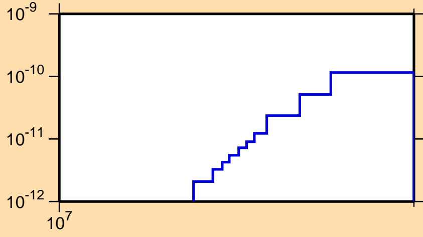
\sigma vs. E for ^{244}\text{Bk}(n,p\alpha)
