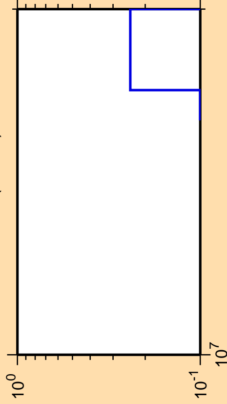
\Delta\sigma/\sigma vs. E for ^{244}\text{Bk} (mt 34)
