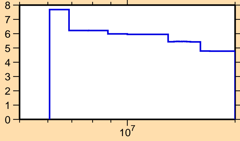
\Delta\sigma/\sigma vs. E for ^{244}\text{Bk}(n,\text{nonel.})
