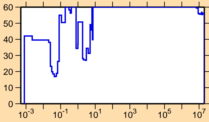
\Delta\sigma/\sigma vs. E for ^{244}\text{Bk}(n,\gamma)
