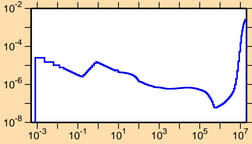
\sigma vs. E for ^{244}\text{Bk}(n,\alpha)
