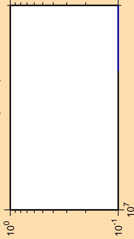
\Delta\sigma/\sigma vs. E for ^{244}\text{Bk} (mt 11)
