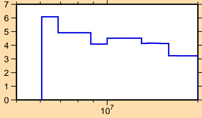
\Delta\sigma/\sigma vs. E for ^{244}\text{Bk}(n,\text{tot.})
