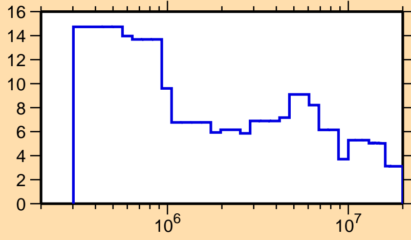
\Delta\sigma/\sigma vs. E for ^{244}\text{Bk}(n,\text{el.})
