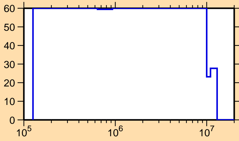
\Delta\sigma/\sigma vs. E for ^{244}\text{Bk}(n,n_1)
