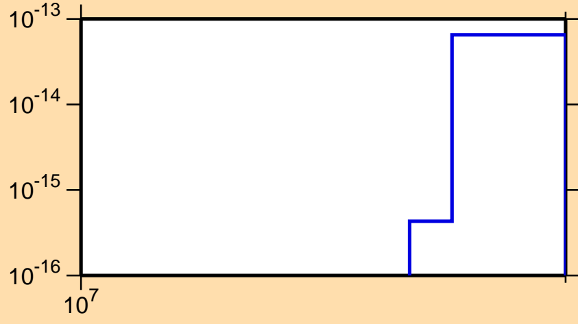
\sigma vs. E for ^{244}\text{Bk} (mt 34)
