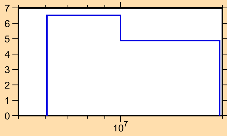
\Delta\sigma/\sigma vs. E for ^{244}\text{Bk}(n,\text{el.})
