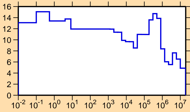
\Delta\sigma/\sigma vs. E for ^{244}\text{Bk}(n,el.)
