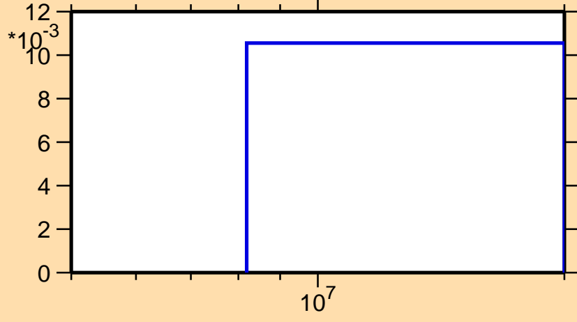
\sigma vs. E for ^{244}\text{Bk}(n,3n)
