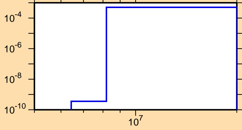
\sigma vs. E for ^{244}\text{Bk}(n,np)
