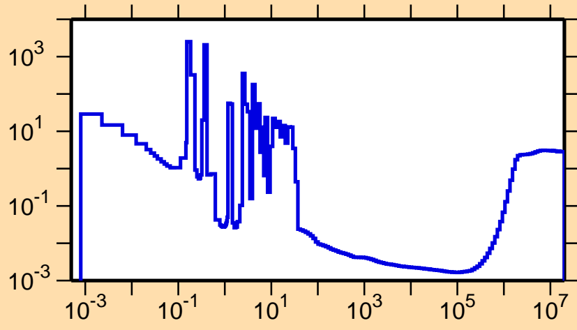
\sigma vs. E for ^{245}\text{Bk}(n,f)
