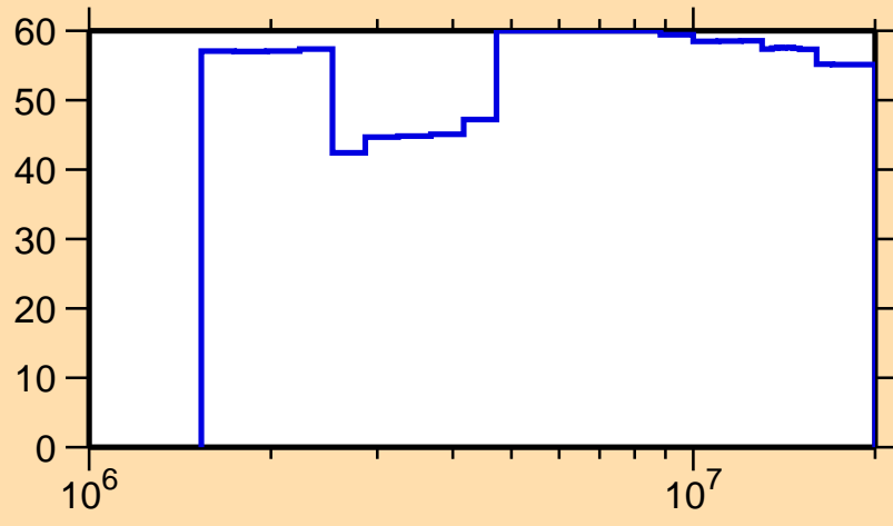
\Delta\sigma/\sigma vs. E for ^{245}\text{Bk}(n,n_1)
