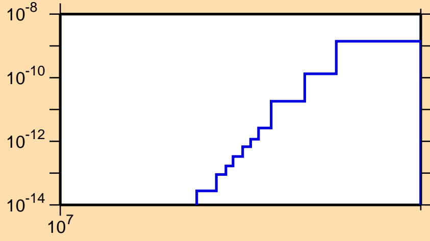
\sigma vs. E for ^{245}\text{Bk}(n,\text{He3})
