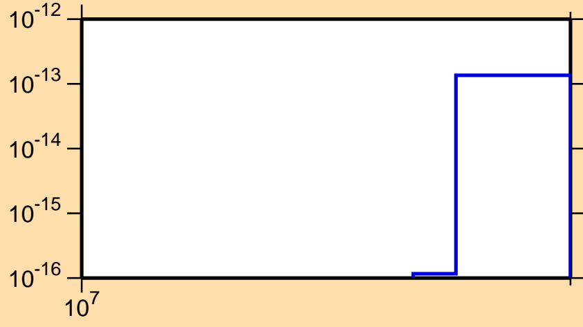
\sigma vs. E for ^{245}\text{Bk} (mt 11)
