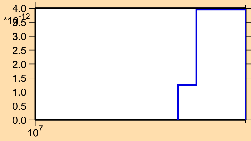
\sigma vs. E for ^{245}\text{Bk}(n,p\alpha)
