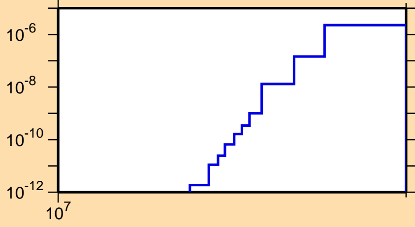
\sigma vs. E for ^{245}\text{Bk}(n,nd)
