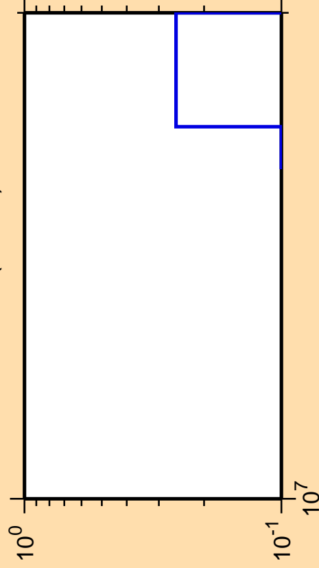
\Delta\sigma/\sigma vs. E for ^{245}\text{Bk} (mt 11)
