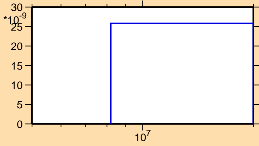
\sigma vs. E for ^{245}\text{Bk}(n,nd)
