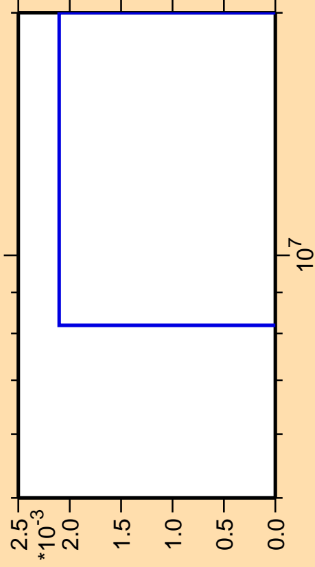
\Delta\sigma/\sigma vs. E for ^{245}\text{Bk}(\text{mt } 11)
