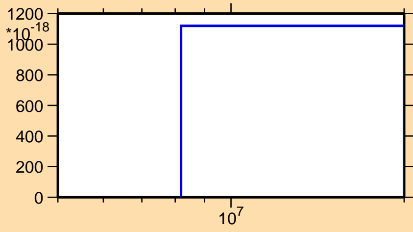
\sigma vs. E for ^{245}\text{Bk}(\text{mt } 11)
