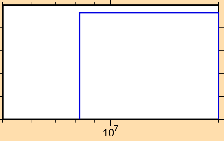
\sigma vs. E for ^{245}\text{Bk}(n,nt)
