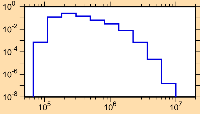
\sigma vs. E for ^{246}\text{Bk}(n,n_1)
