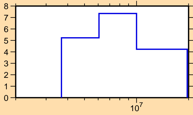
\Delta\sigma/\sigma vs. E for ^{246}\text{Bk}(n,\text{tot.})
