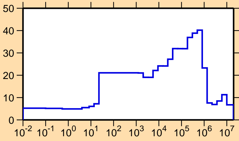
\Delta\sigma/\sigma vs. E for ^{246}\text{Bk}(n,el.)
