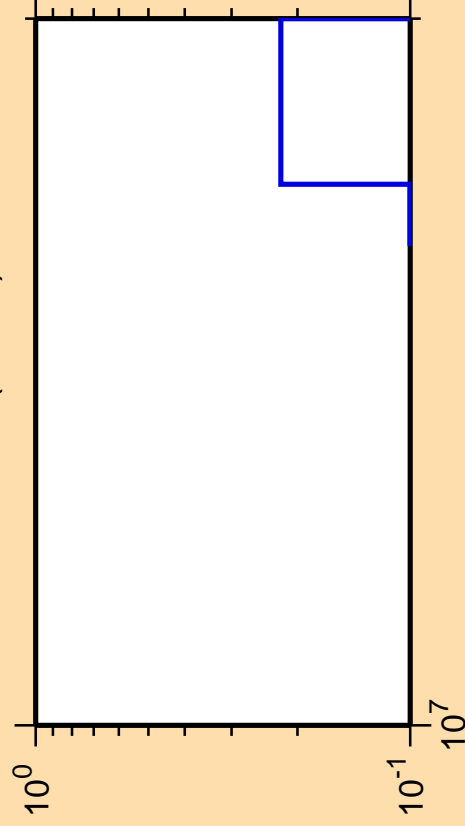
\Delta\sigma/\sigma vs. E for ^{247}\text{Bk} (mt 11)
