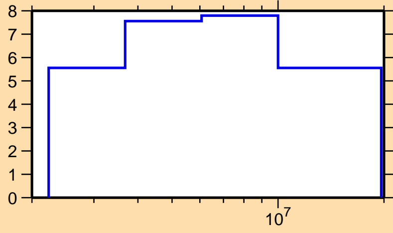
\Delta\sigma/\sigma vs. E for ^{247}\text{Bk}(n,el.)
