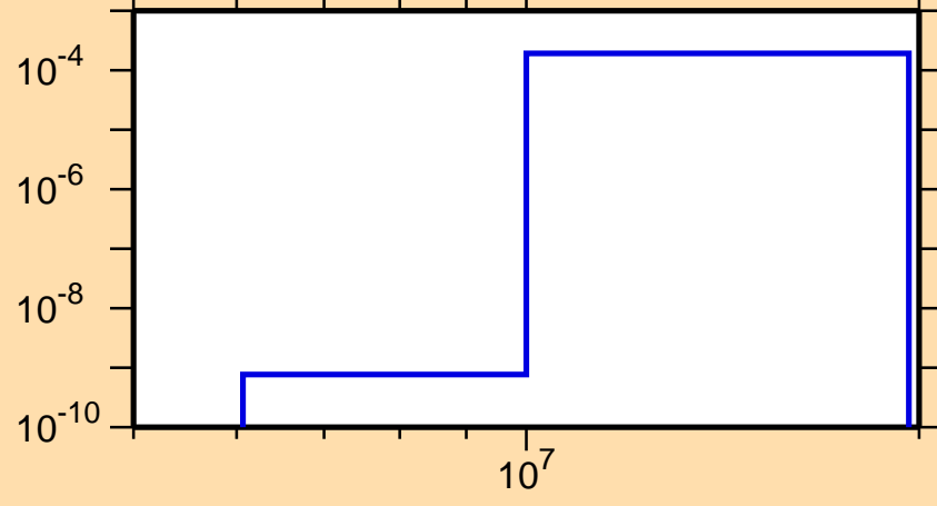
\sigma vs. E for ^{247}\text{Bk}(n,np)
