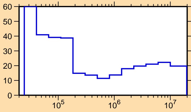
\Delta\sigma/\sigma vs. E for ^{247}\text{Bk}(n,n_1)
