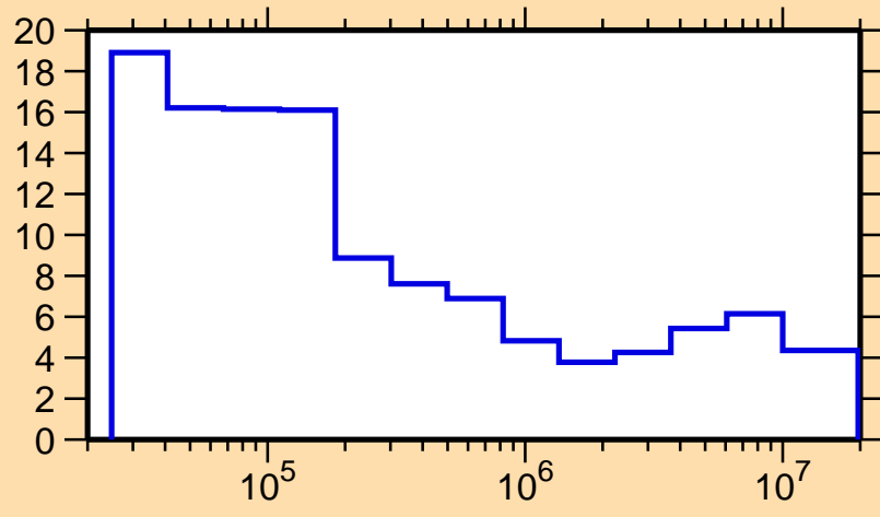
\Delta\sigma/\sigma vs. E for ^{247}\text{Bk}(n,\text{tot.})
