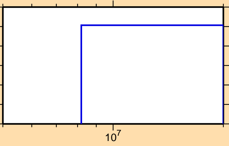
\sigma vs. E for ^{247}\text{Bk}(n,nt)
