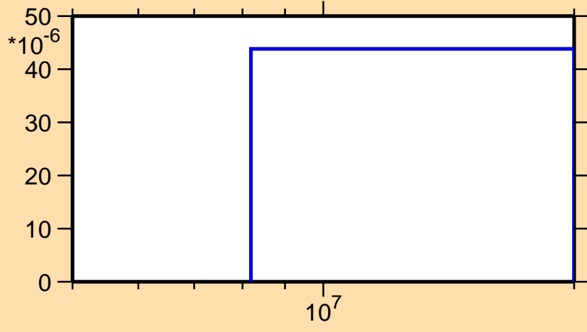
\sigma vs. E for ^{247}\text{Bk}(n,t)
