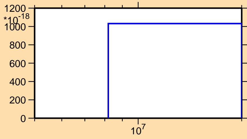
\sigma vs. E for ^{247}\text{Bk} (mt 11)
