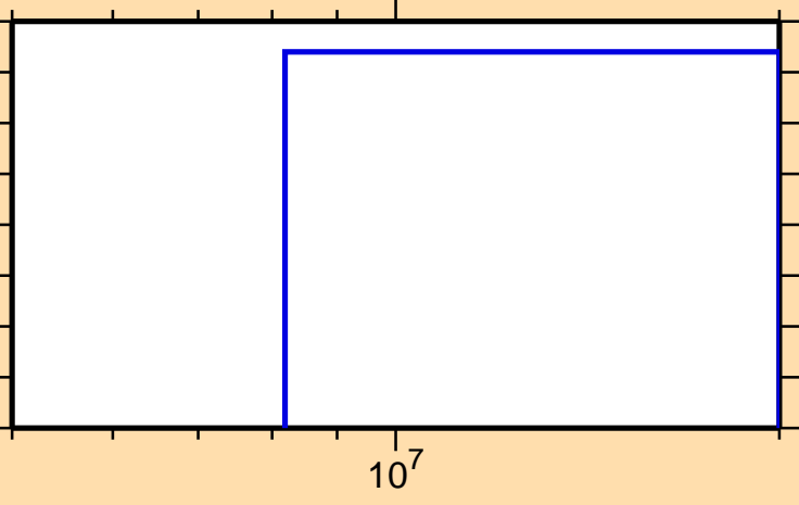
\sigma vs. E for ^{247}\text{Bk}(n,nd)
