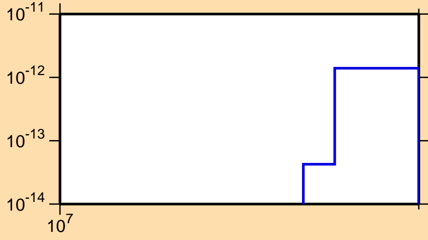
\sigma vs. E for ^{248}\text{Bk}(n,3n\alpha)
