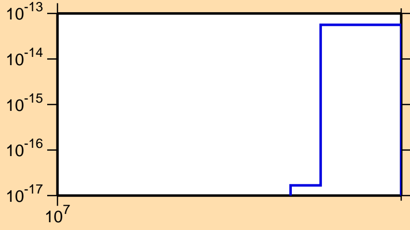
\sigma vs. E for ^{248}\text{Bk} (mt 11)
