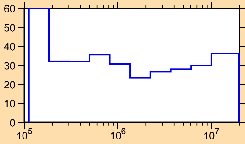
\Delta\sigma/\sigma vs. E for ^{248}\text{Bk}(n,n_1)
