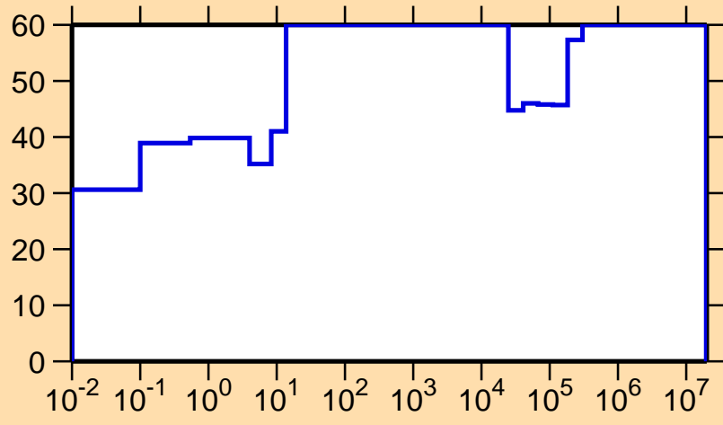
\Delta\sigma/\sigma vs. E for ^{248}\text{Bk}(n,\gamma)
