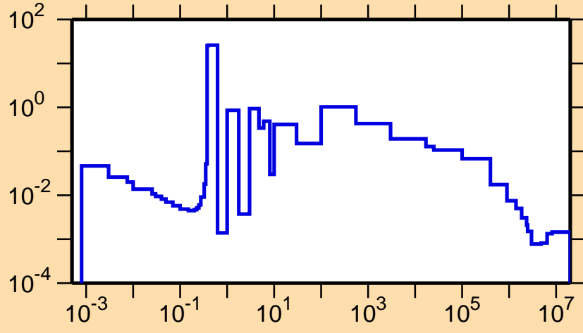
\sigma vs. E for ^{248}\text{Bk}(n,\gamma)
