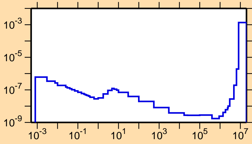
\sigma vs. E for ^{248}\text{Bk}(n,\alpha)
