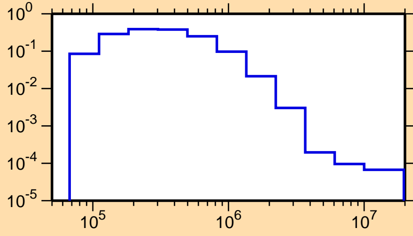
\sigma vs. E for ^{249}\text{Bk}(n,n_4)
