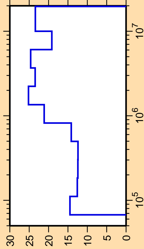
\Delta\sigma/\sigma vs. E for ^{249}\text{Bk}(n,n_4)
