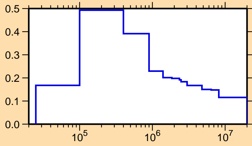
\sigma vs. E for ^{249}\text{Bk}(n,n_3)
