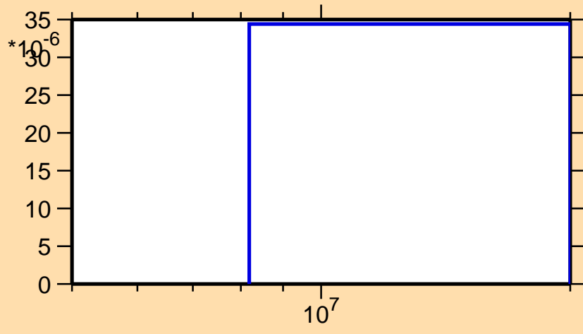
\sigma vs. E for ^{249}\text{Bk}(n,t)
