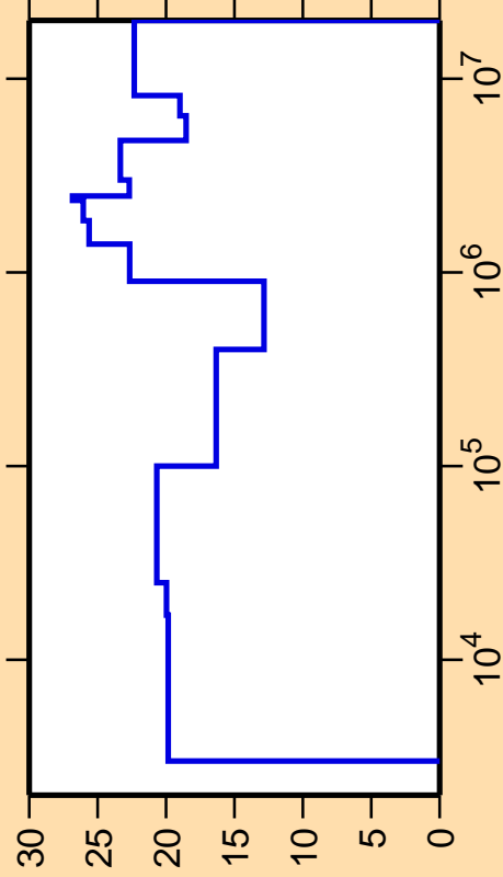
\Delta\sigma/\sigma vs. E for ^{249}\text{Bk}(n,n_1)
