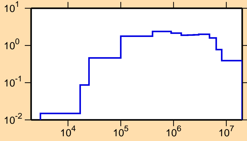
\sigma vs. E for ^{249}\text{Bk}(n,\text{inel.})
