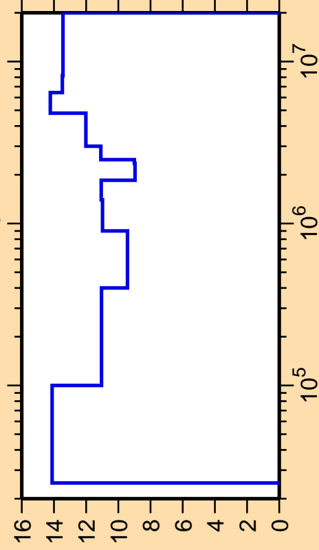
\Delta\sigma/\sigma vs. E for ^{249}\text{Bk}(n,n_3)
