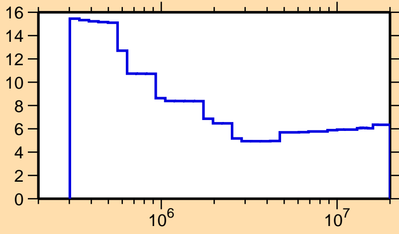
\Delta\sigma/\sigma vs. E for ^{250}\text{Bk}(n,\text{nonel.})
