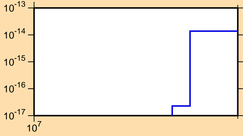
\sigma vs. E for ^{250}\text{Bk} (mt 11)
