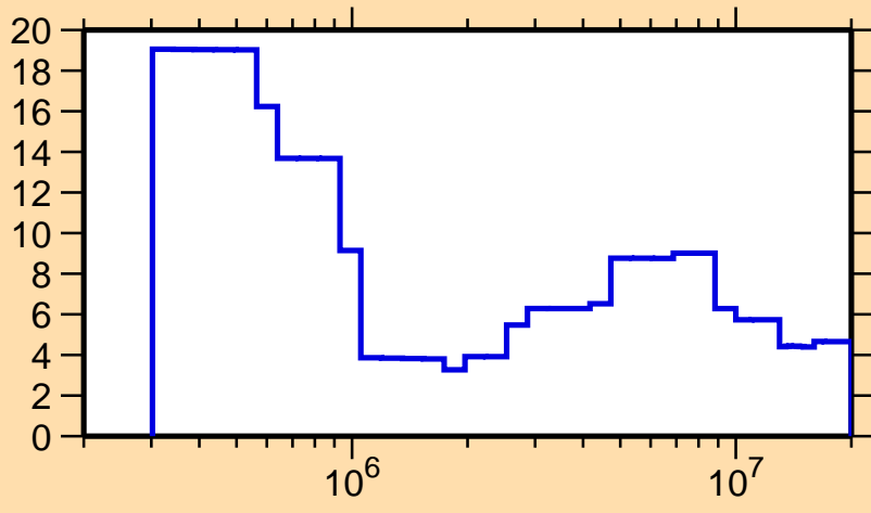
\Delta\sigma/\sigma vs. E for ^{250}\text{Bk}(n,\text{tot.})
