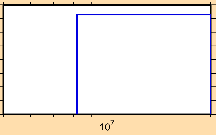
\sigma vs. E for ^{250}\text{Bk}(n,nt)
