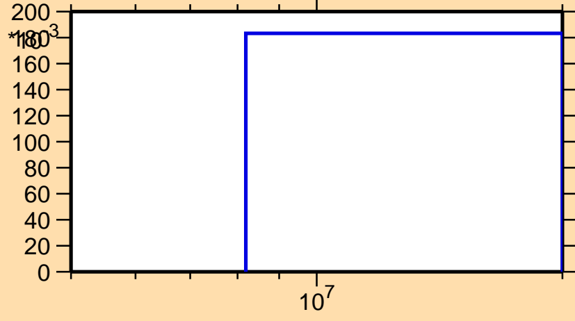
\sigma vs. E for ^{250}\text{Bk}(n,3n)
