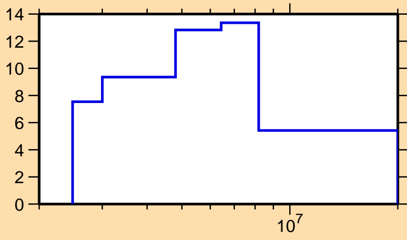
\Delta\sigma/\sigma vs. E for ^{250}\text{Bk}(n,el.)
