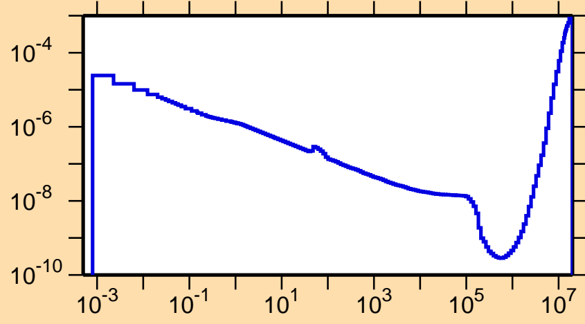
\sigma vs. E for ^{252}\text{Bk}(n,\alpha)
