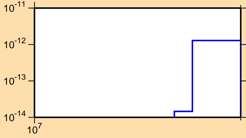
\sigma vs. E for ^{252}\text{Bk}(n,3n\alpha)
