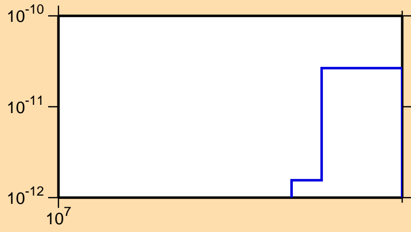
\sigma vs. E for ^{252}\text{Bk}(n,\text{He3})
