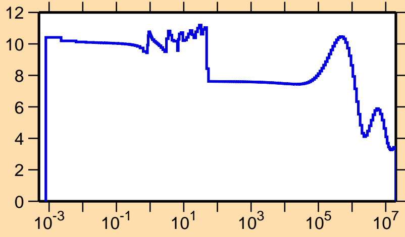
\sigma vs. E for ^{252}\text{Bk}(n,\text{el.})
