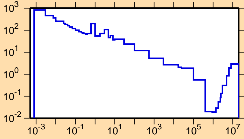
\sigma vs. E for ^{252}\text{Bk}(n,f)
