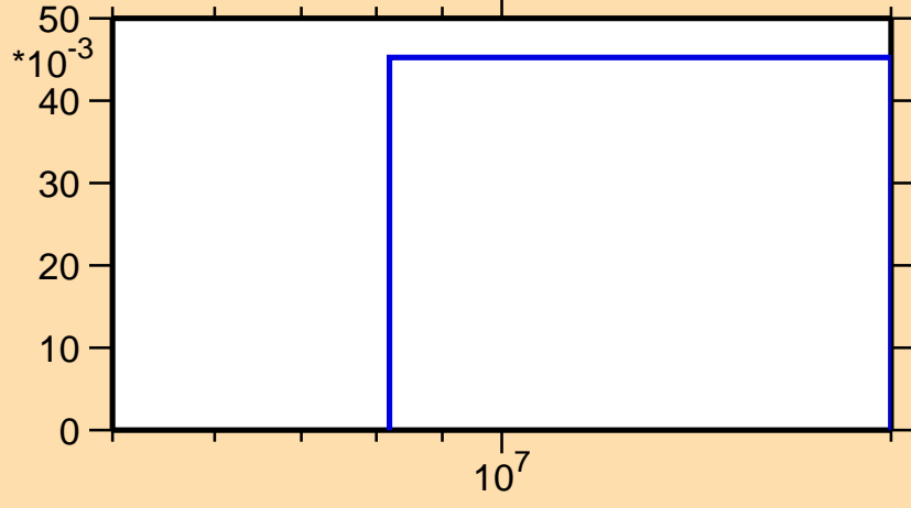
\sigma vs. E for ^{252}\text{Bk}(n,3n)
