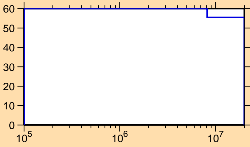
\Delta\sigma/\sigma vs. E for ^{252}\text{Bk}(n,n_1)
