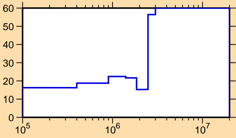
\Delta\sigma/\sigma vs. E for ^{252}\text{Bk}(n,n\text{cont.})
