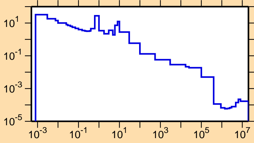
\sigma vs. E for ^{252}\text{Bk}(n,\gamma)
