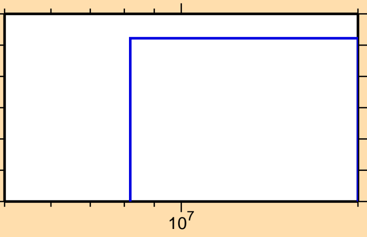
\sigma vs. E for ^{252}\text{Bk}(n,nt)
