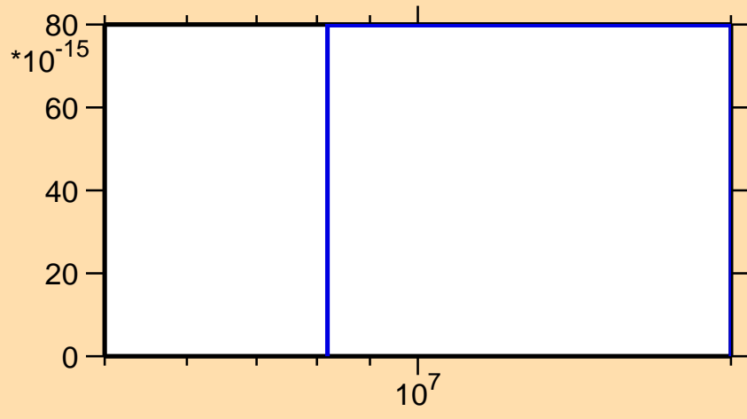
\sigma vs. E for ^{252}\text{Bk} (mt 11)
