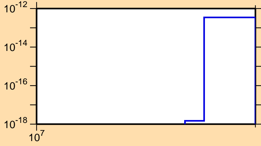
\sigma vs. E for ^{253}\text{Bk} (mt 11)
