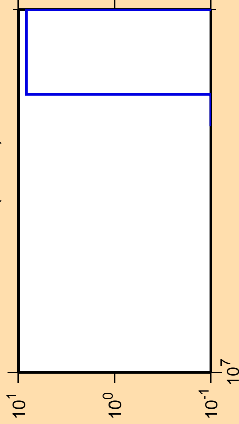
\Delta\sigma/\sigma vs. E for ^{254}\text{Bk} (mt 11)
