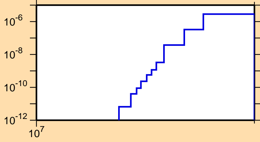
\sigma vs. E for ^{254}\text{Bk}(n,nd)
