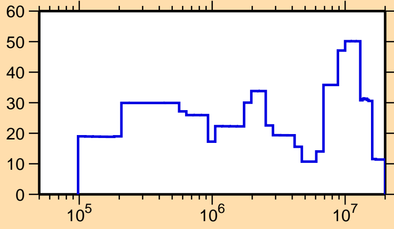
\Delta\sigma/\sigma vs. E for ^{254}\text{Bk}(n, tot.)
