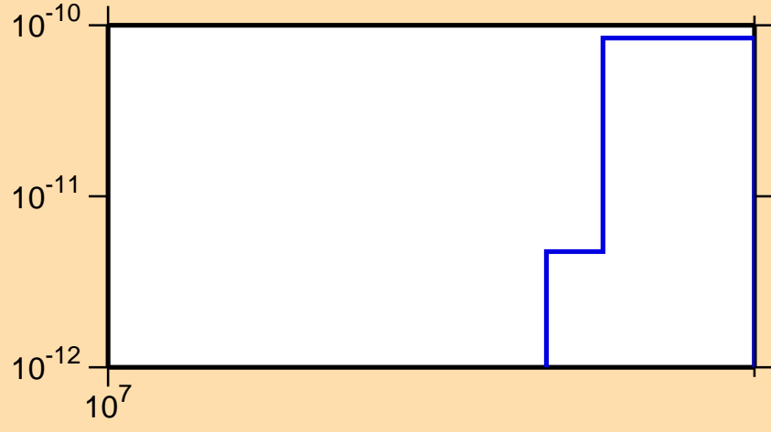
\sigma vs. E for ^{254}\text{Bk}(n,\text{He3})
