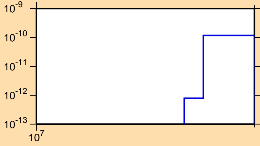
\sigma vs. E for ^{254}\text{Bk}(n,3n\alpha)
