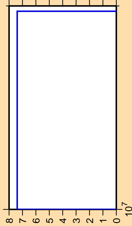
\Delta\sigma/\sigma vs. E for ^{254}\text{Bk}(n,3n\alpha)
