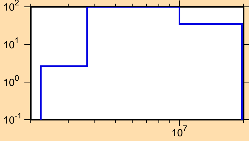
\Delta\sigma/\sigma vs. E for ^{254}\text{Bk}(n,p)
