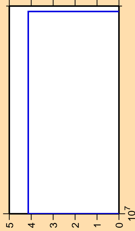
\Delta\sigma/\sigma vs. E for ^{254}\text{Bk}(n,\text{He3})
