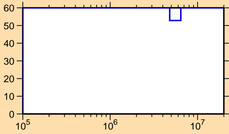
\Delta\sigma/\sigma vs. E for ^{254}\text{Bk}(n,n\text{cont.})
