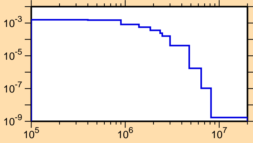
\sigma vs. E for ^{254}\text{Bk}(n,n_1)
