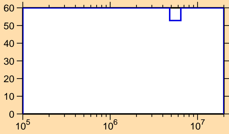
\Delta\sigma/\sigma vs. E for ^{254}\text{Bk}(n,\text{inel.})
