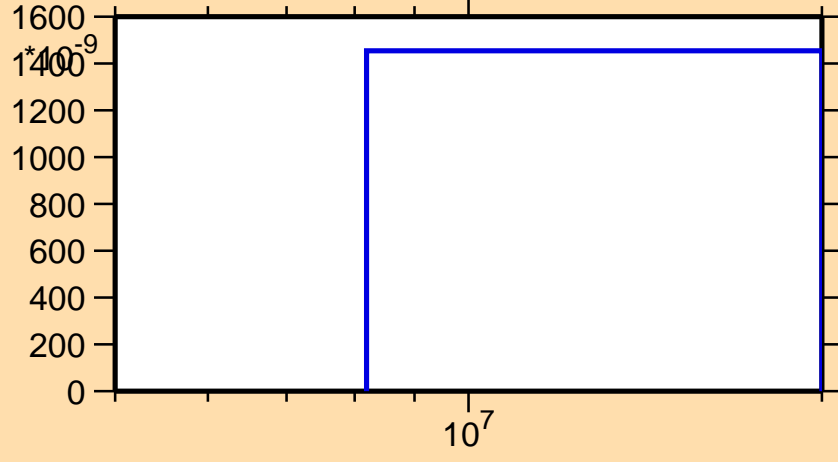
\sigma vs. E for ^{254}\text{Bk}(n,np)
