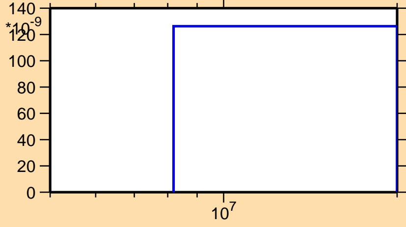
\sigma vs. E for ^{254}\text{Bk}(n,nt)
