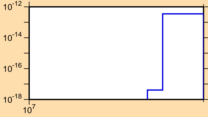
\sigma vs. E for ^{70}\text{Br}(n,2n\alpha)
