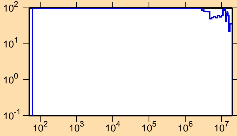
\Delta\sigma/\sigma vs. E for ^{70}\text{Br}(n,n_1)
