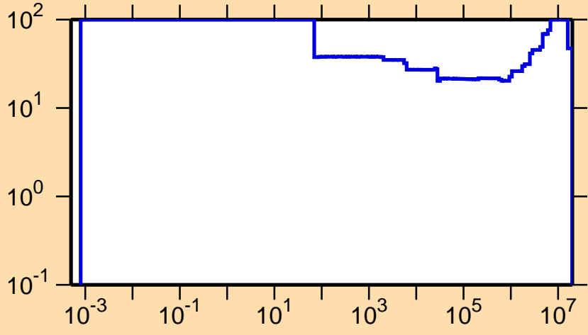
\Delta\sigma/\sigma vs. E for ^{70}\text{Br}(n,p)
