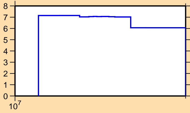
\Delta\sigma/\sigma vs. E for ^{70}\text{Br}(n,\text{el.})
