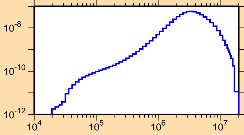
\sigma vs. E for ^{70}\text{Br}(n,n_1)
