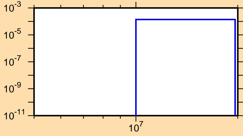
\sigma vs. E for ^{70}\text{Br}(n,pt)
