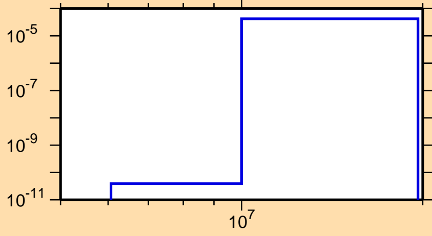
\sigma vs. E for ^{70}\text{Br} (mt 45)
