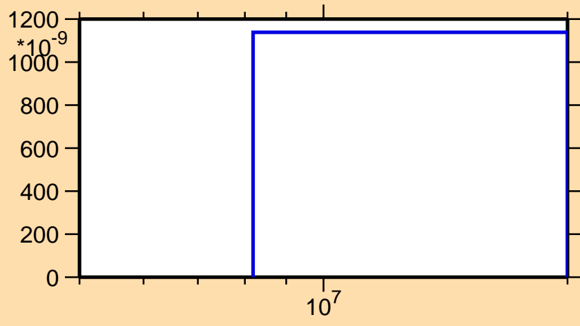
\sigma vs. E for ^{70}\text{Br}(n,2np)
