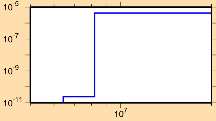
\sigma vs. E for ^{70}\text{Br}(\text{mt117})
