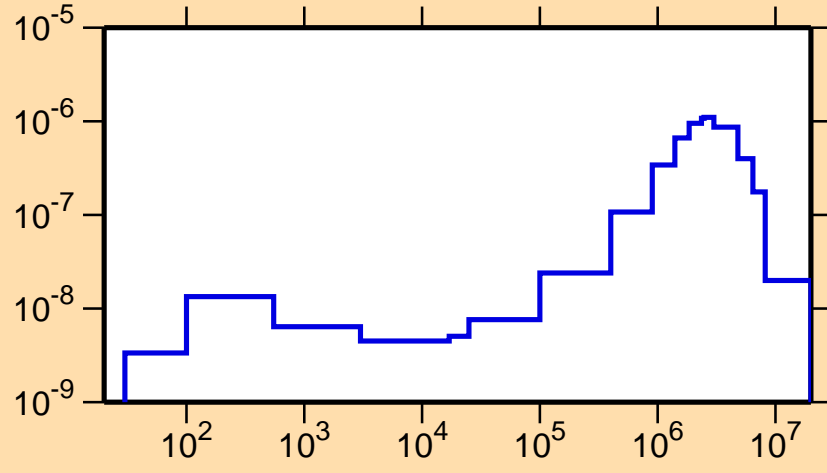
\sigma vs. E for ^{70}\text{Br}(n,n_2)
