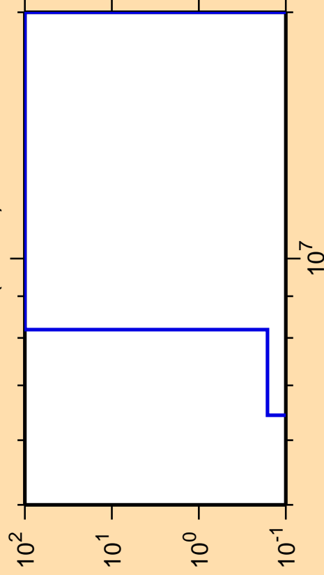
\Delta\sigma/\sigma vs. E for ^{70}\text{Br} (mt 45)
