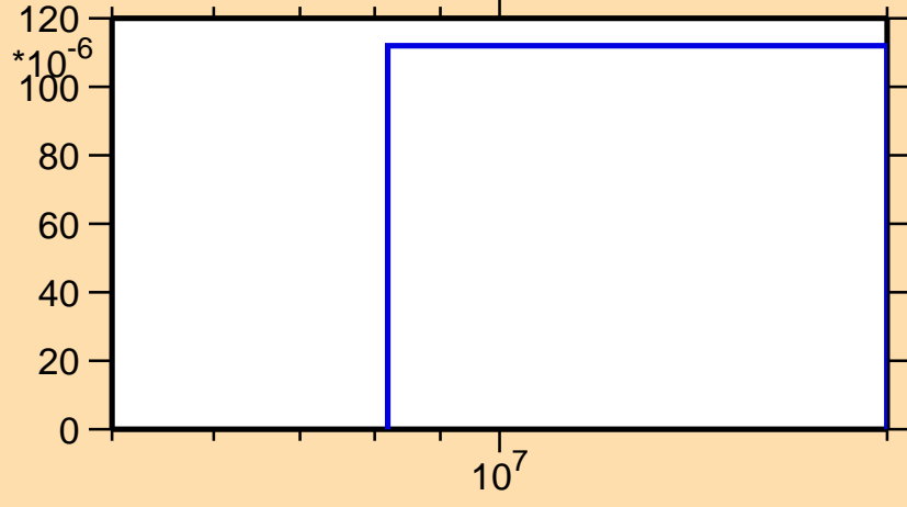
\sigma vs. E for ^{70}\text{Br}(n,\text{pt})
