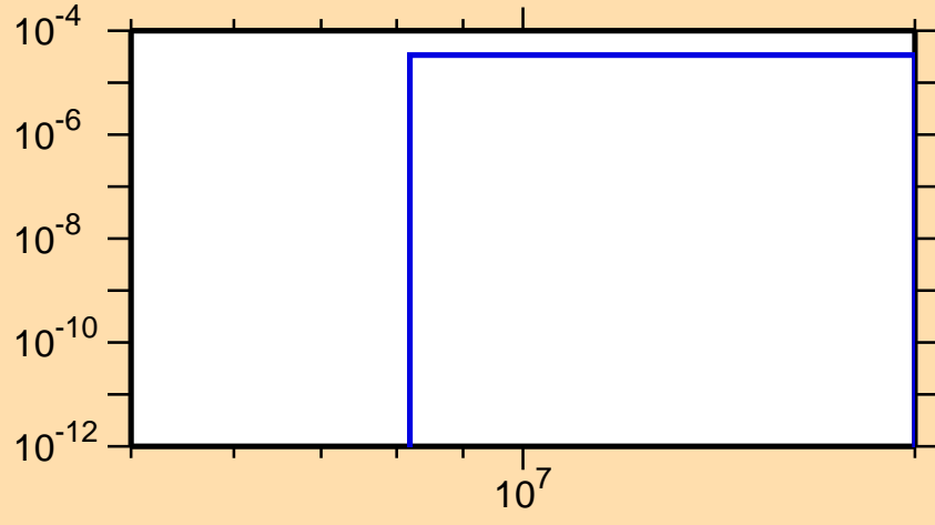
\sigma vs. E for ^{70}\text{Br} (mt 45)
