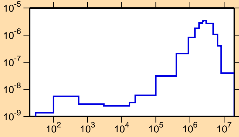
\sigma vs. E for ^{70}\text{Br}(n,n_3)
