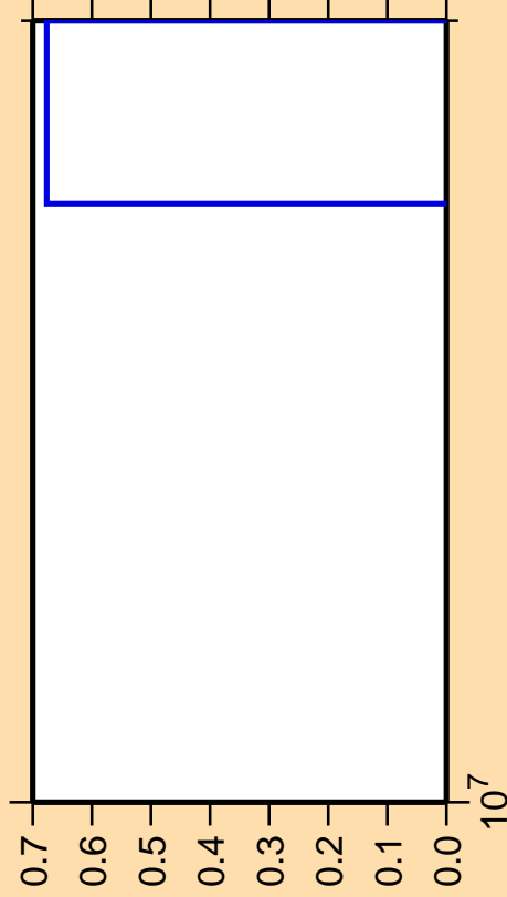
\Delta\sigma/\sigma vs. E for ^{71}\text{Br}(n,nt)
