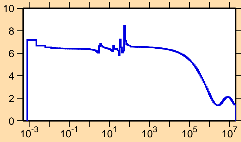
\sigma vs. E for ^{71}\text{Br}(n,\text{el.})
