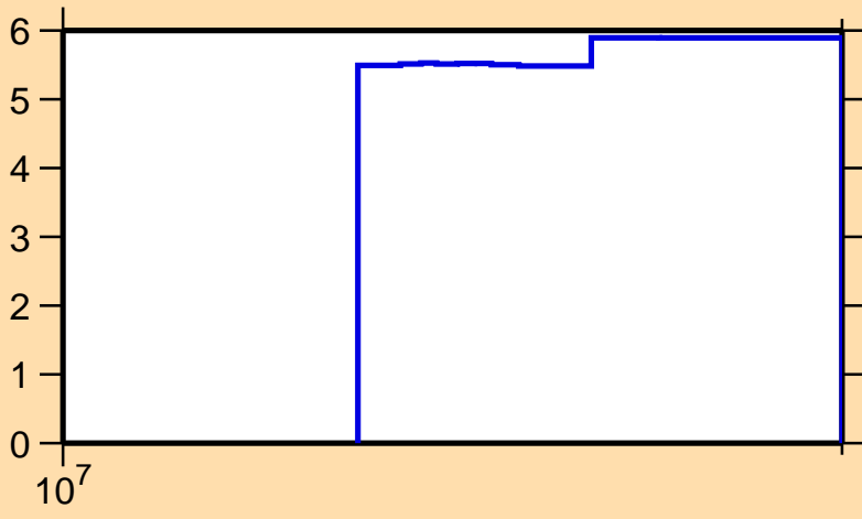
\Delta\sigma/\sigma vs. E for ^{71}\text{Br}(n,\text{nonel.})
