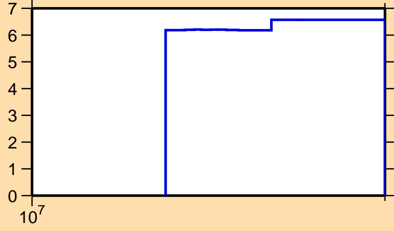
\Delta\sigma/\sigma vs. E for ^{71}\text{Br}(n,\text{tot.})
