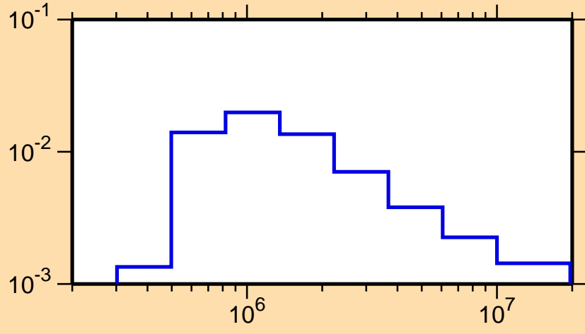
\sigma vs. E for ^{71}\text{Br}(n,n_3)
