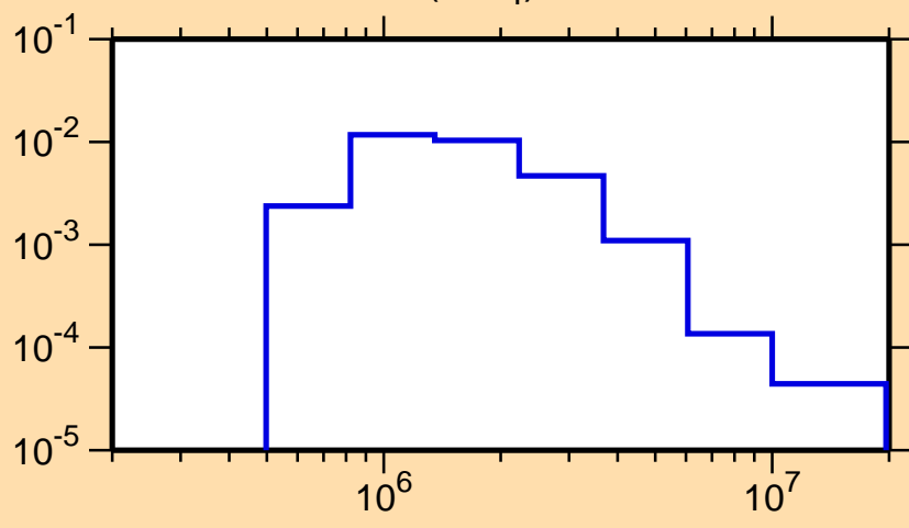
\sigma vs. E for ^{71}\text{Br}(n,n_4)
