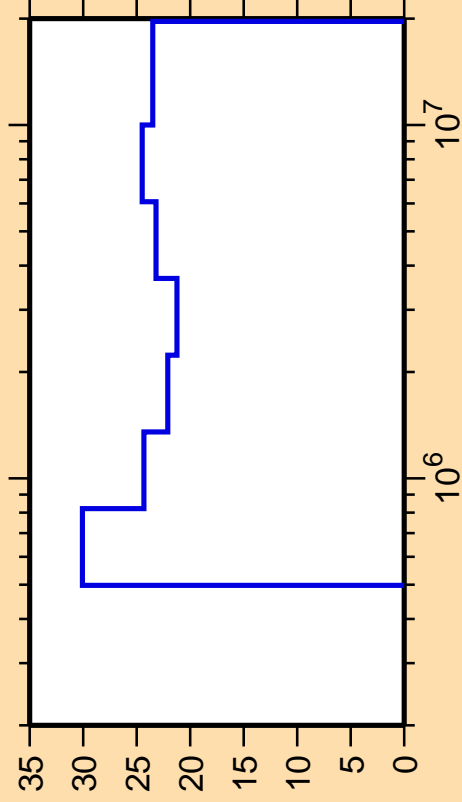
\Delta\sigma/\sigma vs. E for ^{71}\text{Br}(n,n_4)
