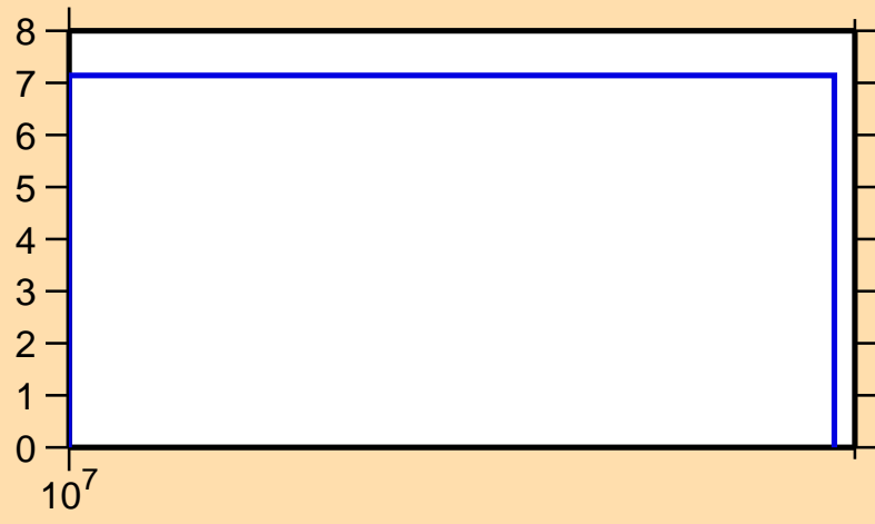
\Delta\sigma/\sigma vs. E for ^{71}\text{Br}(n,\text{el.})
