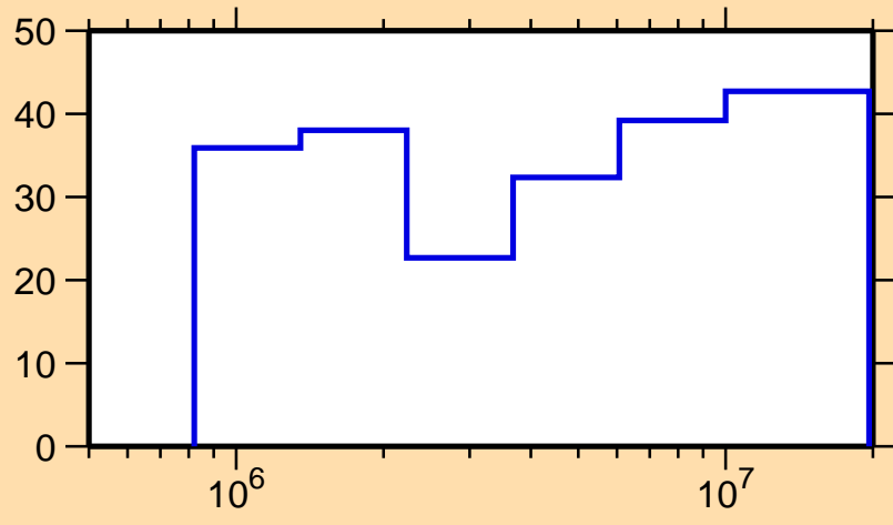
\Delta\sigma/\sigma vs. E for ^{71}\text{Br}(n,ncont.)
