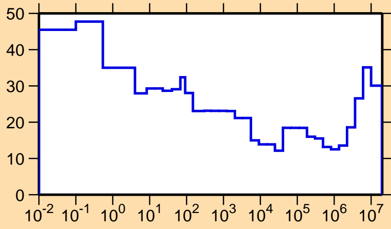
\Delta\sigma/\sigma vs. E for ^{71}\text{Br}(n,p)
