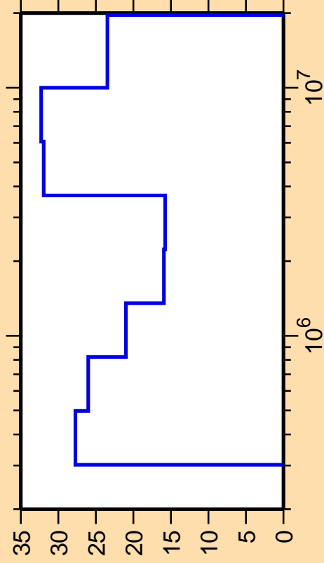
\Delta\sigma/\sigma vs. E for ^{71}\text{Br}(n,n_3)
