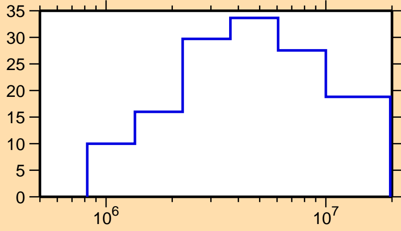
\Delta\sigma/\sigma vs. E for ^{71}\text{Br}(n,inel.)
