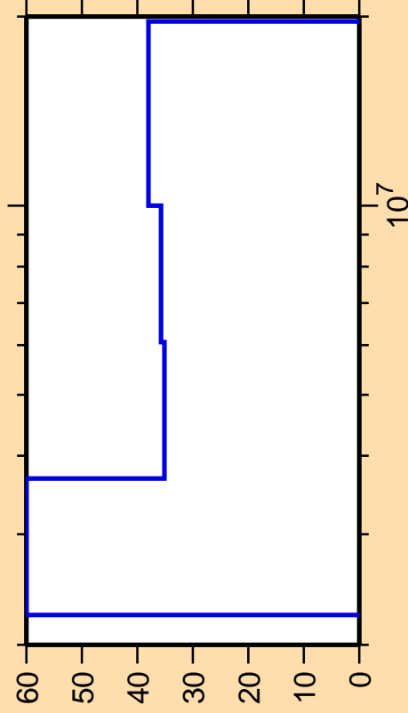
\Delta\sigma/\sigma vs. E for ^{71}\text{Br}(n,np)
