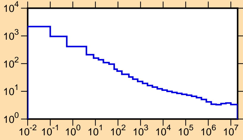
\sigma vs. E for ^{71}\text{Br}(n,\text{tot.})
