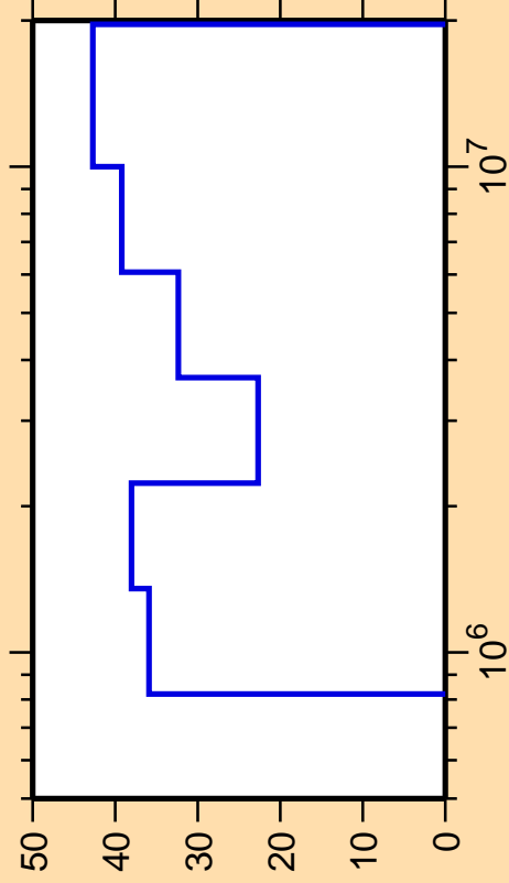
\Delta\sigma/\sigma vs. E for ^{71}\text{Br}(n,ncont.)
