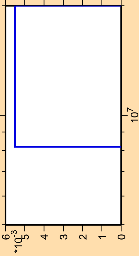
\Delta\sigma/\sigma vs. E for ^{71}\text{Br}(n,nt)
