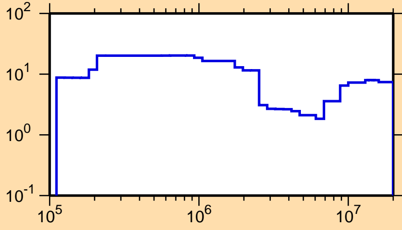
\Delta\sigma/\sigma vs. E for ^{72}\text{Br}(n,tot.)
