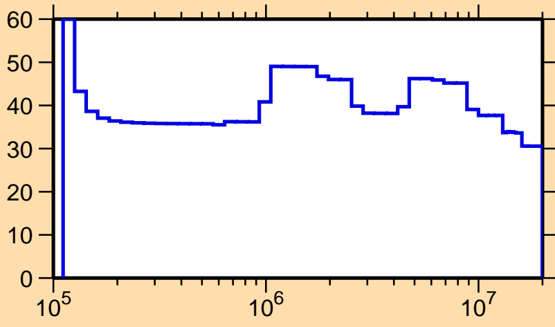
\Delta\sigma/\sigma vs. E for ^{72}\text{Br}(n,n_1)
