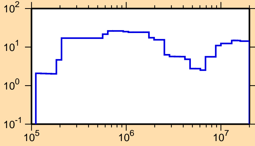
\Delta\sigma/\sigma vs. E for ^{72}\text{Br}(n,el.)
