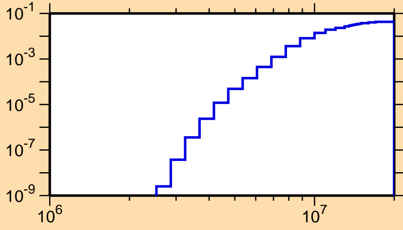
\sigma vs. E for ^{72}\text{Br}(n,d)
