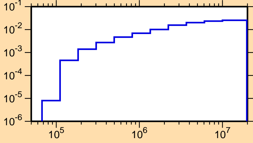
\sigma vs. E for ^{72}\text{Br}(n,n_1)
