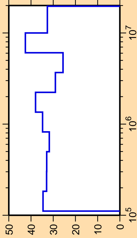
\Delta\sigma/\sigma vs. E for ^{72}\text{Br}(n,n_2)
