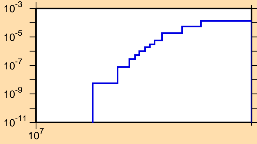
\sigma vs. E for ^{72}\text{Br}(n,nd)
