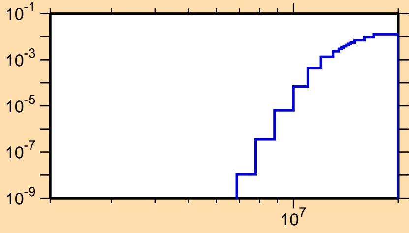
\sigma vs. E for ^{72}\text{Br}(n, n\alpha)
