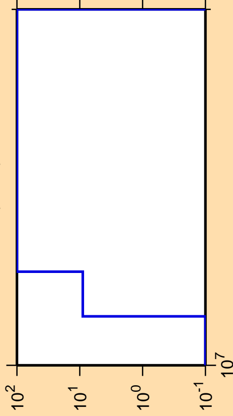
\Delta\sigma/\sigma vs. E for ^{72}\text{Br}(n,nd)
