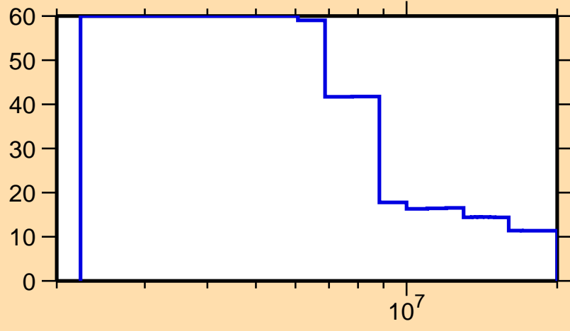
\Delta\sigma/\sigma vs. E for ^{73}\text{Br}(n,ncont.)
