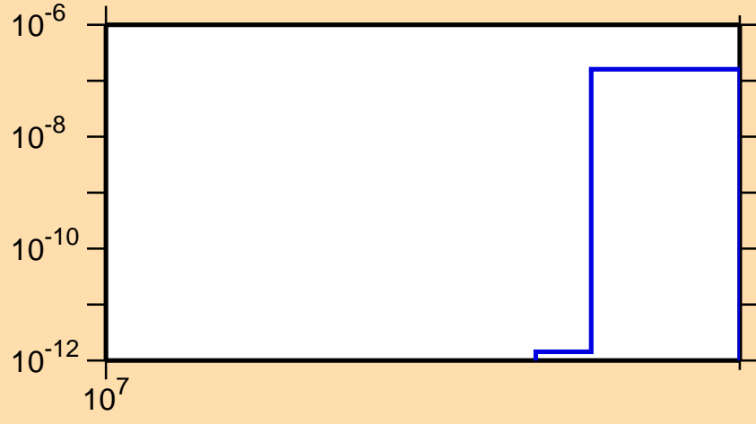
\sigma vs. E for ^{73}\text{Br}(n,\text{pt})
