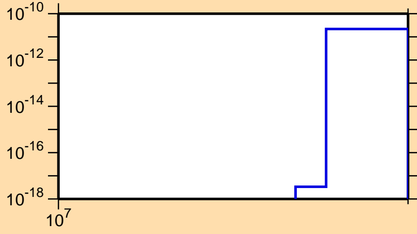
\sigma vs. E for ^{73}\text{Br} (mt 34)
