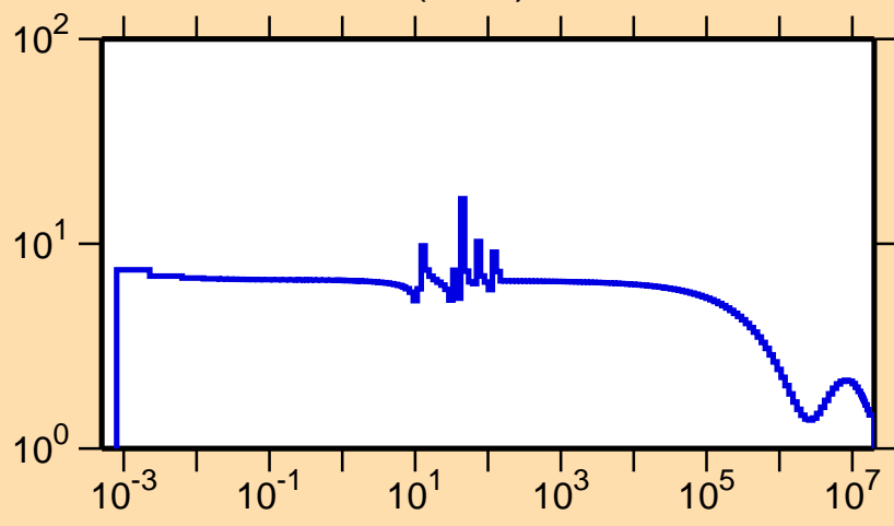
\sigma vs. E for ^{73}\text{Br}(n,\text{el.})
