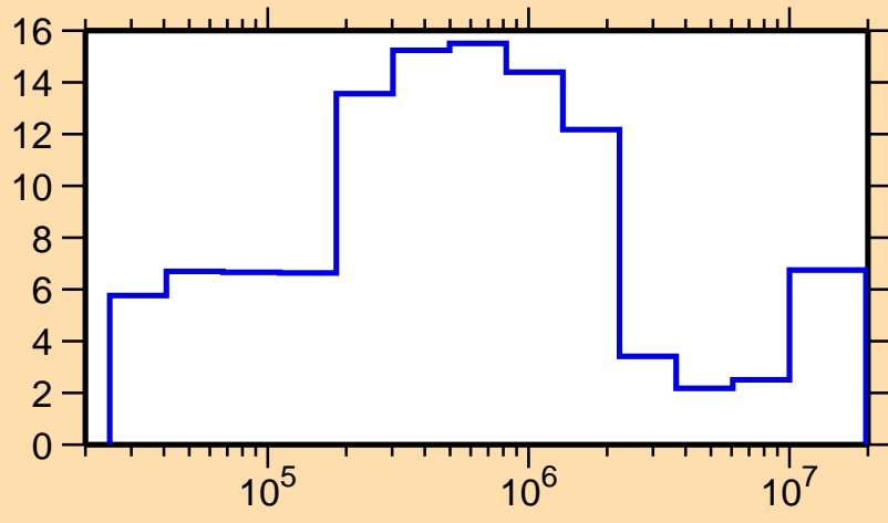
\Delta\sigma/\sigma vs. E for ^{73}\text{Br}(n,\text{tot.})
