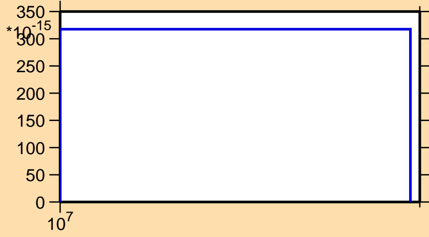
\sigma vs. E for ^{73}\text{Br}(n,nt)
