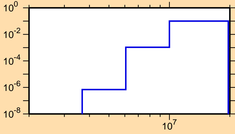
\sigma vs. E for ^{73}\text{Br}(n,p\alpha)
