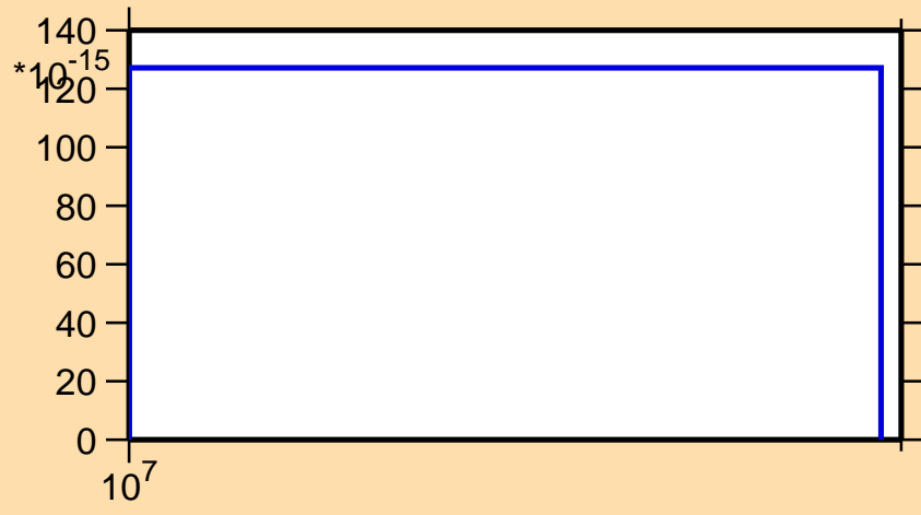
\sigma vs. E for ^{73}\text{Br} (mt 34)
