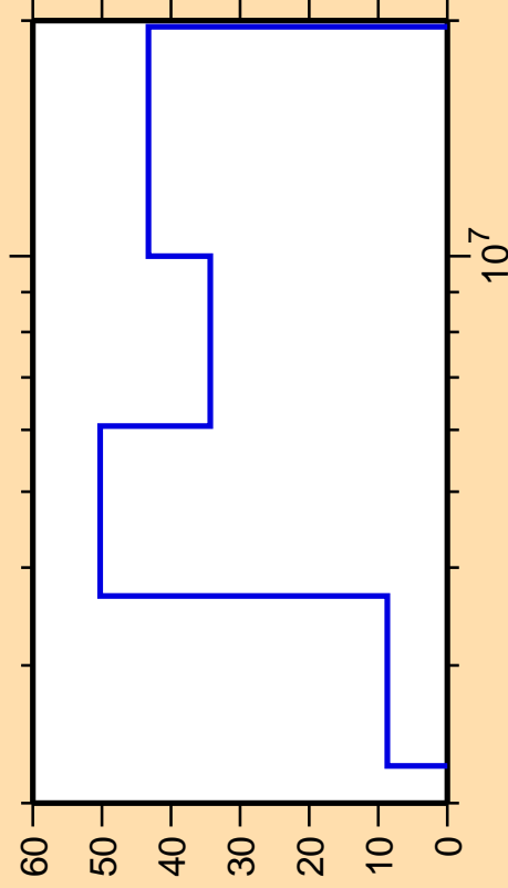
\Delta\sigma/\sigma vs. E for ^{73}\text{Br}(n,p\alpha)
