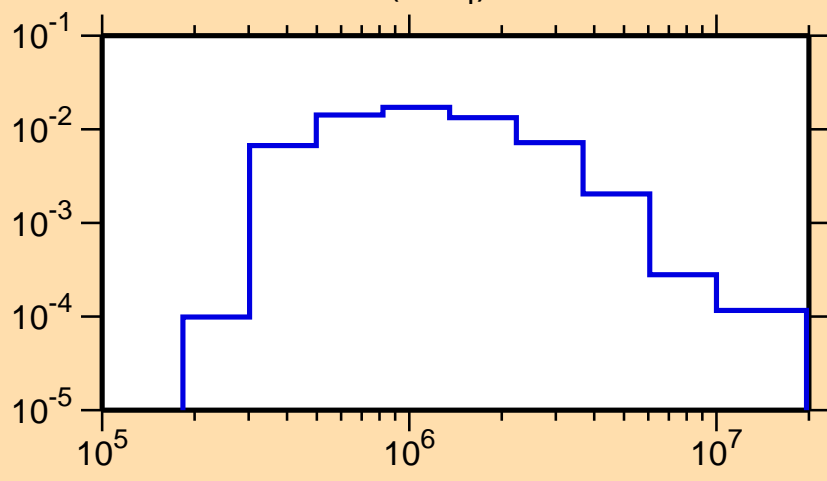
\sigma vs. E for ^{73}\text{Br}(n,n_4)
