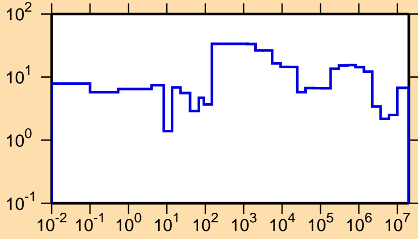
\Delta\sigma/\sigma vs. E for ^{73}\text{Br}(n,\text{tot.})
