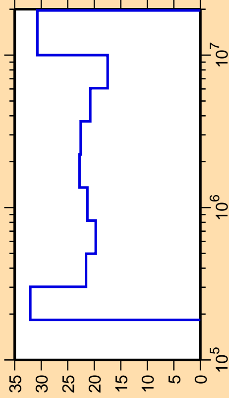
\Delta\sigma/\sigma vs. E for ^{73}\text{Br}(n,n_4)
