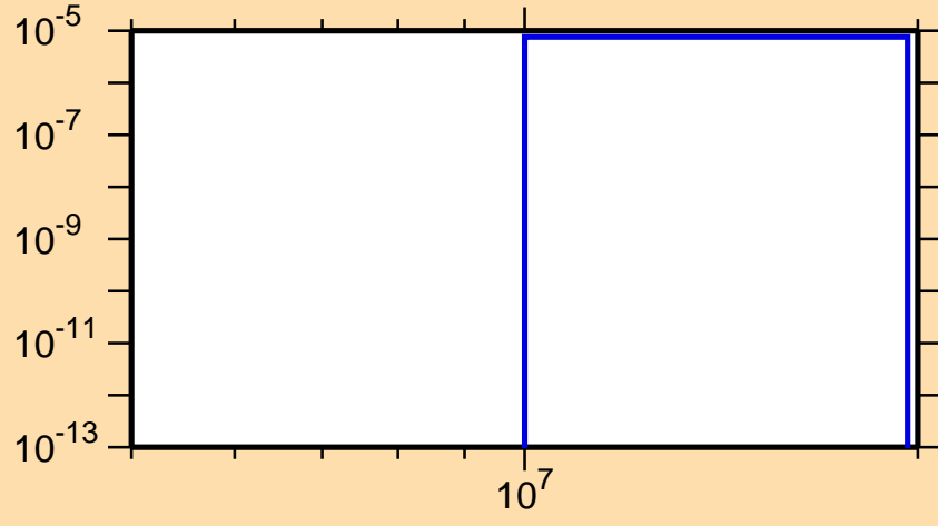
\sigma vs. E for ^{73}\text{Br} (mt 45)
