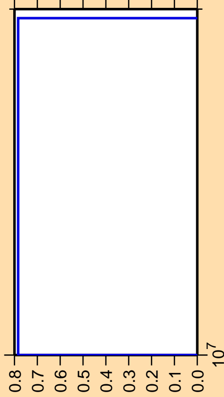
\Delta\sigma/\sigma vs. E for ^{73}\text{Br} (mt 34)
