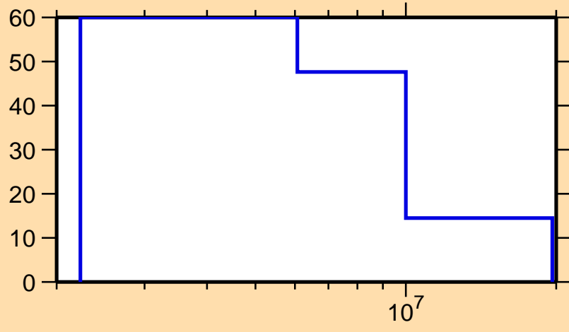
\Delta\sigma/\sigma vs. E for ^{73}\text{Br}(n,n\text{cont.})
