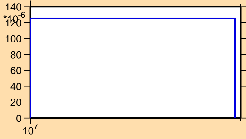
\sigma vs. E for ^{73}\text{Br}(n,\text{pd})
