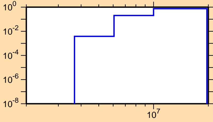
\sigma vs. E for ^{73}\text{Br}(n,np)
