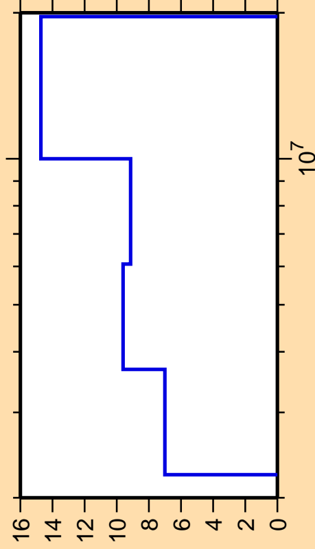
\Delta\sigma/\sigma vs. E for ^{73}\text{Br}(n,p)
