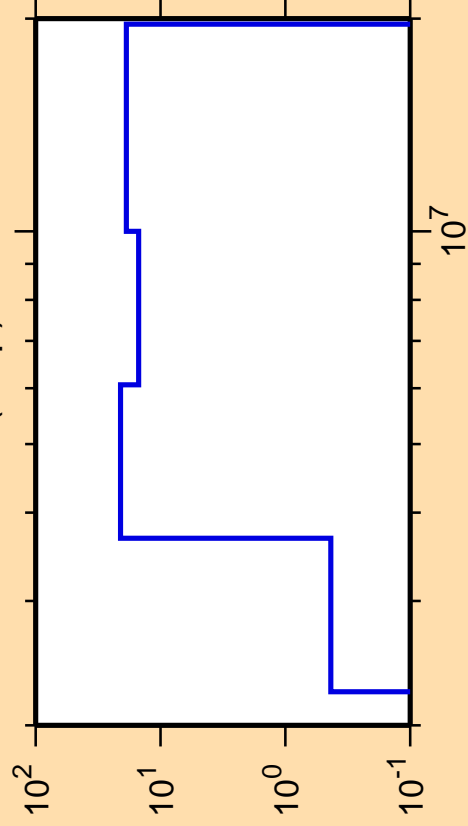
\Delta\sigma/\sigma vs. E for ^{73}\text{Br}(n,np)
