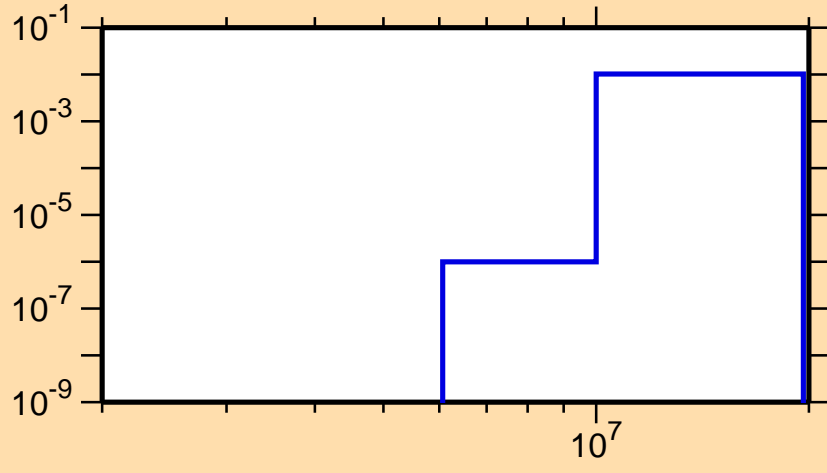
\sigma vs. E for ^{73}\text{Br}(n,n\alpha)
