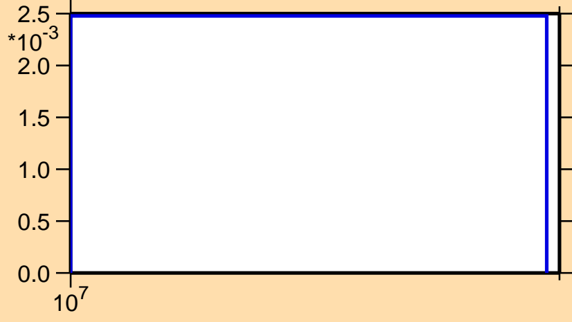
\sigma vs. E for ^{73}\text{Br}(n,2n)
