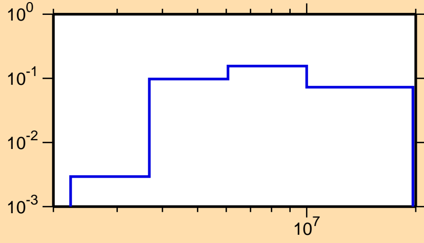
\sigma vs. E for ^{73}\text{Br}(n,n\text{cont.})
