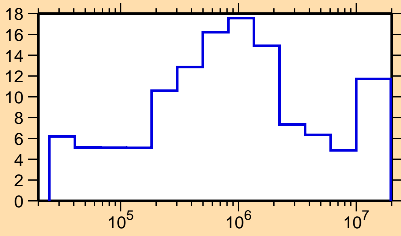
\Delta\sigma/\sigma vs. E for ^{73}\text{Br}(n,\text{el.})
