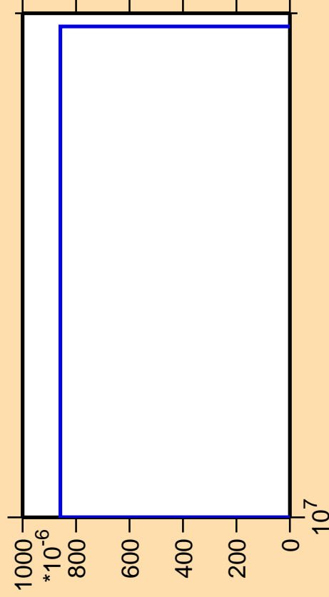
\Delta\sigma/\sigma vs. E for ^{73}\text{Br}(n,2n\alpha)
