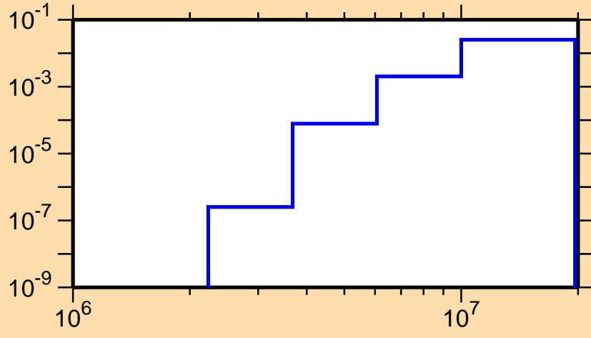
\sigma vs. E for ^{73}\text{Br}(n,d)
