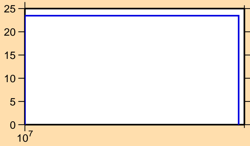
\Delta\sigma/\sigma vs. E for ^{73}\text{Br}(n,\text{inel.})
