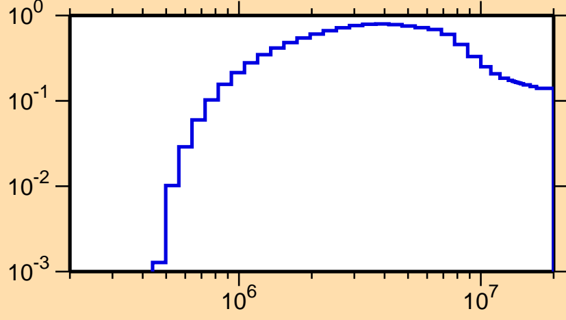
\sigma vs. E for ^{74}\text{Br}(n,n\text{cont.})
