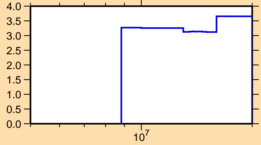
\Delta\sigma/\sigma vs. E for ^{74}\text{Br}(n,\text{nonel.})
