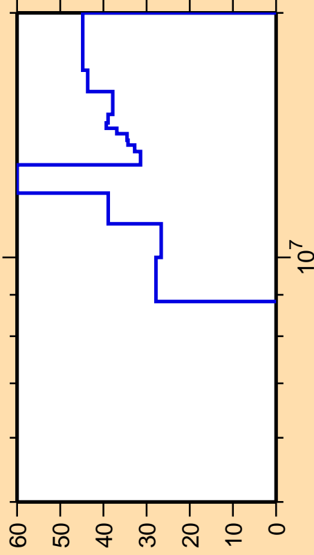
\Delta\sigma/\sigma vs. E for ^{74}\text{Br}(n,n_1)
