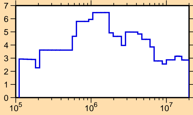
\Delta\sigma/\sigma vs. E for ^{75}\text{Br}(n,\text{el.})
