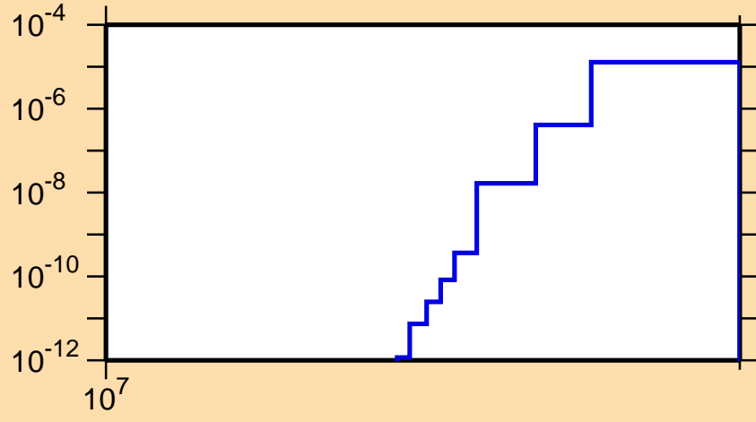
\sigma vs. E for ^{75}\text{Br} (mt 45)
