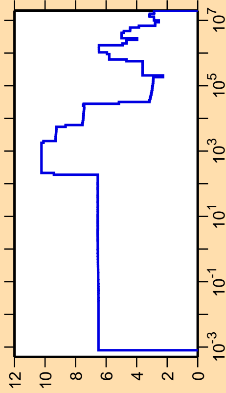
\Delta\sigma/\sigma vs. E for ^{75}\text{Br}(n,\text{el.})
