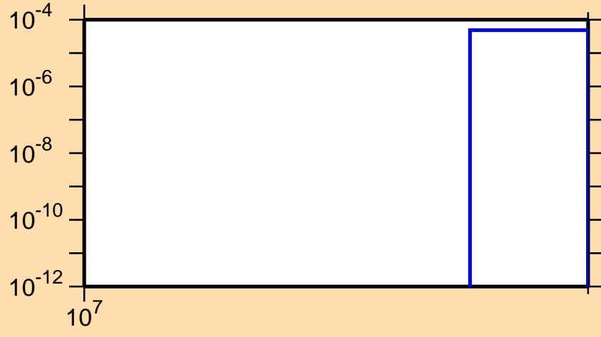
\sigma vs. E for ^{75}\text{Br}(n,2np)
