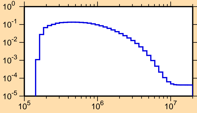
\sigma vs. E for ^{75}\text{Br}(n,n_3)
