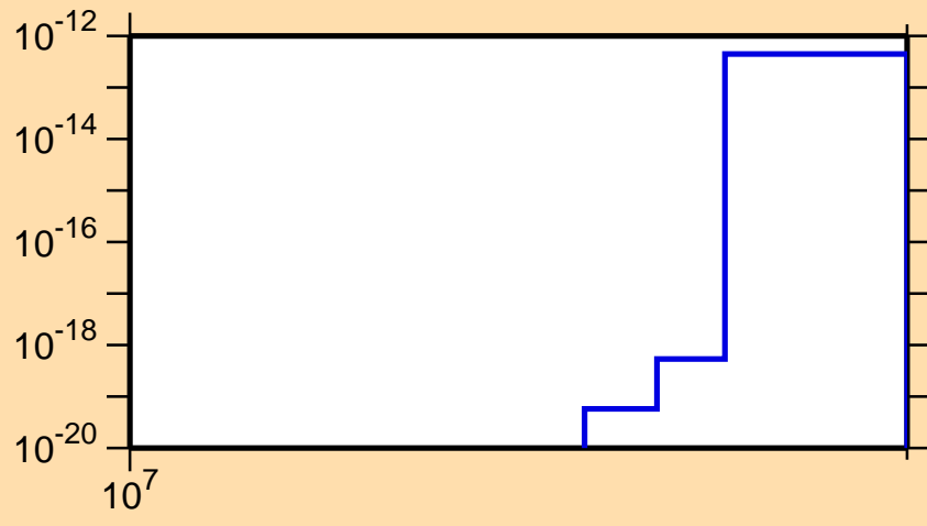
\sigma vs. E for ^{75}\text{Br}(n,2n\alpha)
