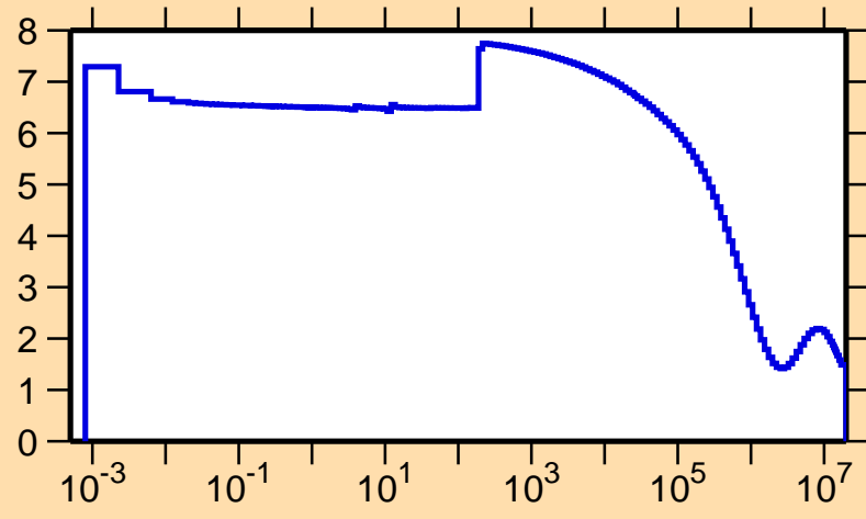
\sigma vs. E for ^{75}\text{Br}(n,\text{el.})
