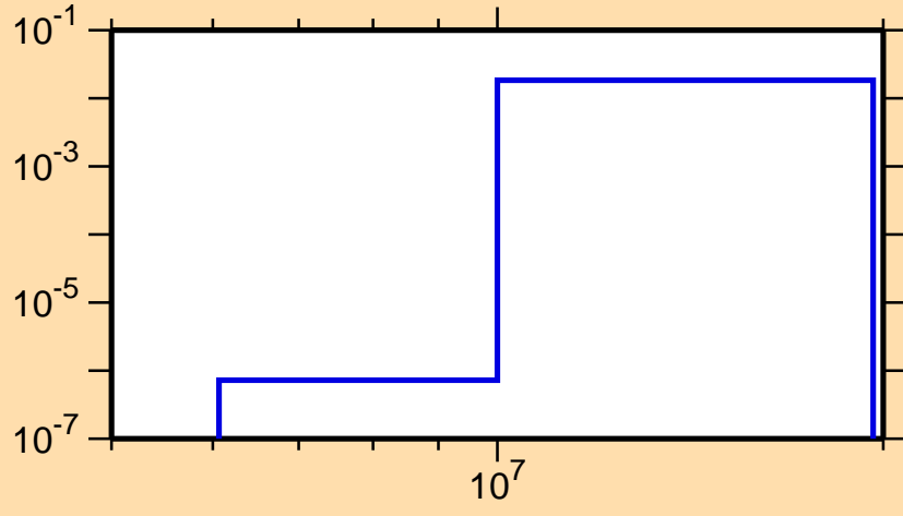
\sigma vs. E for ^{75}\text{Br}(n,n\alpha)
