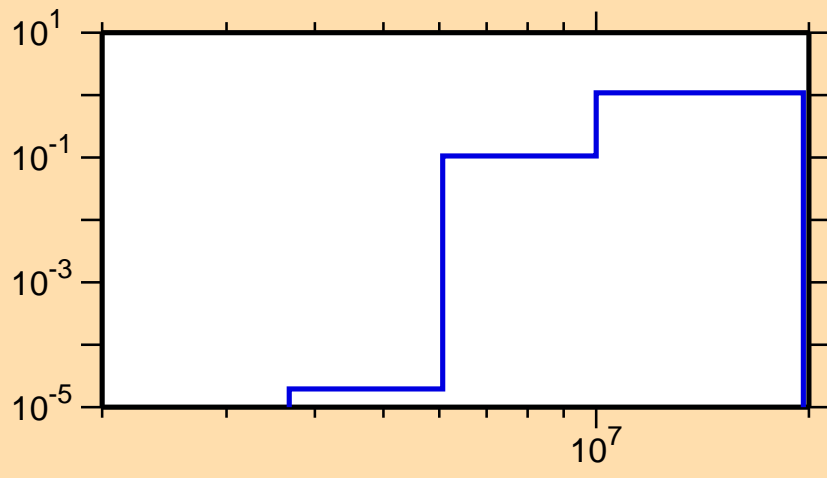
\sigma vs. E for ^{75}\text{Br}(n,np)
