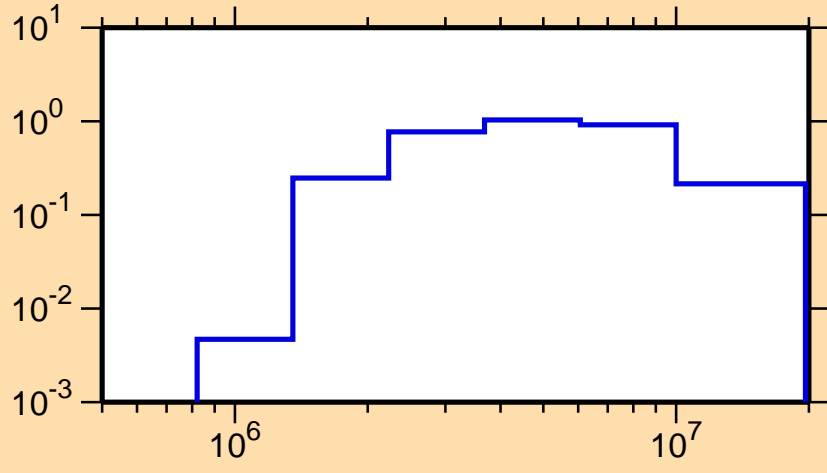
\sigma vs. E for ^{75}\text{Br}(n,n\text{cont.})
