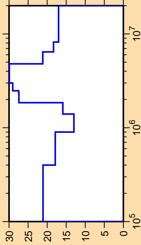
\Delta\sigma/\sigma vs. E for ^{75}\text{Br}(n,n_1)
