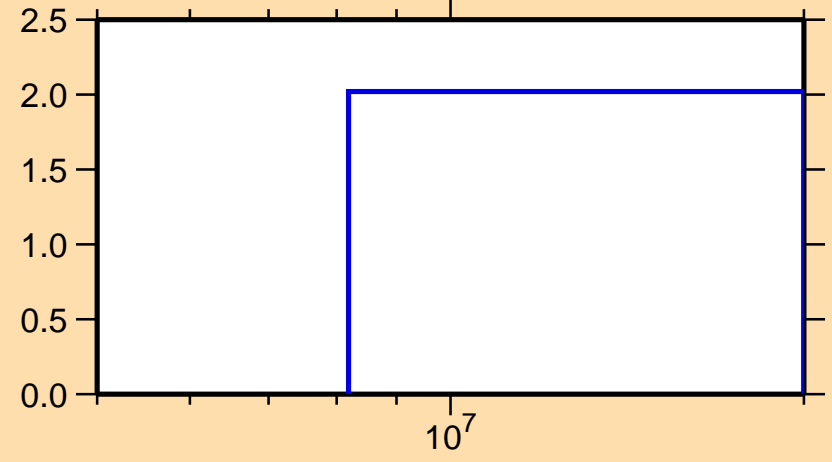
\Delta\sigma/\sigma vs. E for ^{75}\text{Br}(n,\text{tot.})
