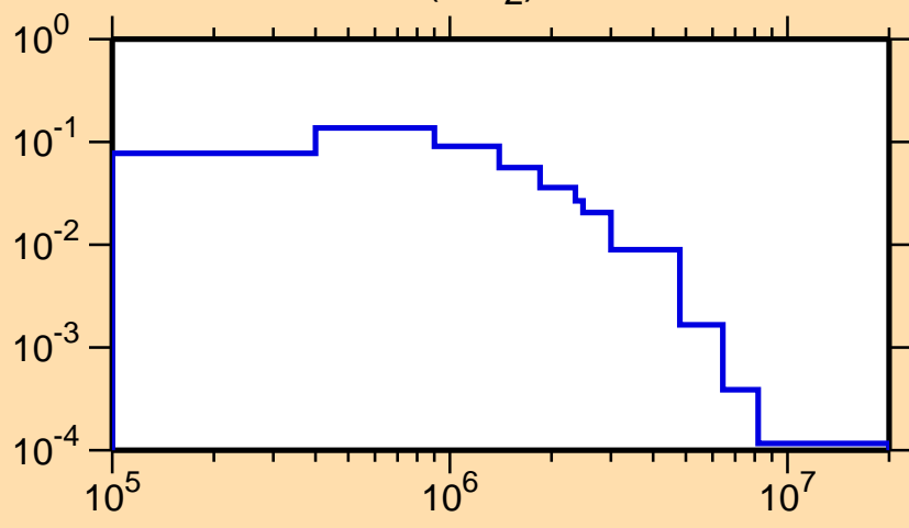
\sigma vs. E for ^{75}\text{Br}(n,n_2)
