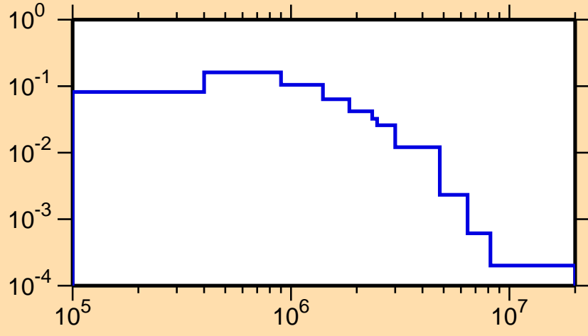
\sigma vs. E for ^{75}\text{Br}(n,n_1)
