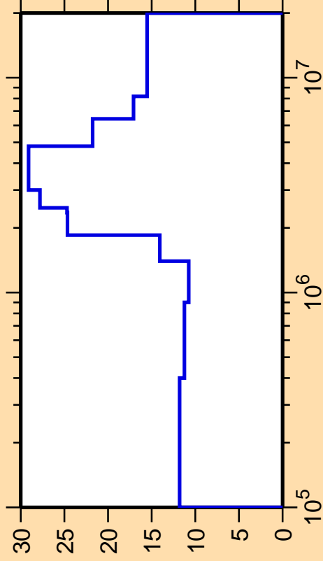
\Delta\sigma/\sigma vs. E for ^{75}\text{Br}(n,n_2)
