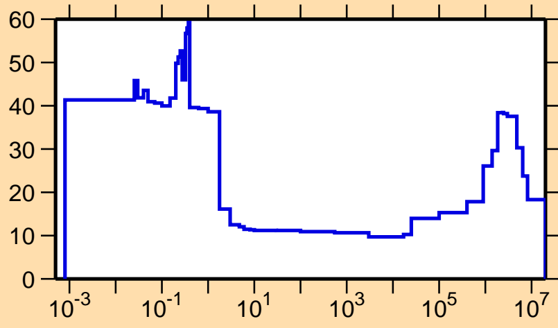
\Delta\sigma/\sigma vs. E for ^{75}\text{Br}(n,p)
