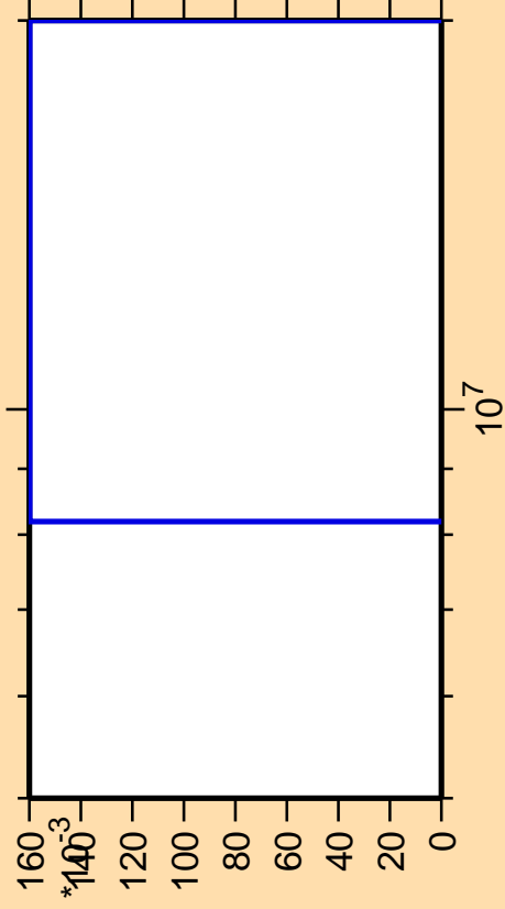
\Delta\sigma/\sigma vs. E for ^{75}\text{Br}(n,\text{pt})
