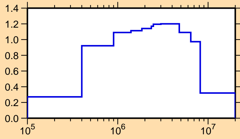
\sigma vs. E for ^{75}\text{Br}(n,\text{inel.})
