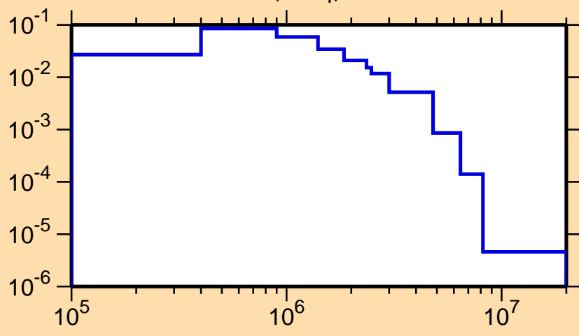
\sigma vs. E for ^{75}\text{Br}(n,n_4)
