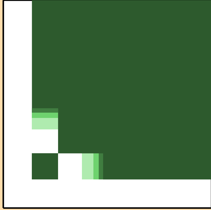
\sigma vs. E for ^{76}\text{Br}(n,nd)
