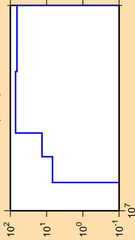
\Delta\sigma/\sigma vs. E for ^{76}\text{Br}(n,nd)
