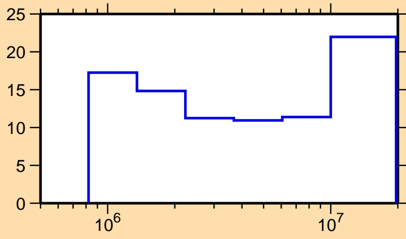
\Delta\sigma/\sigma vs. E for ^{76}\text{Br}(n,n\text{cont.})
