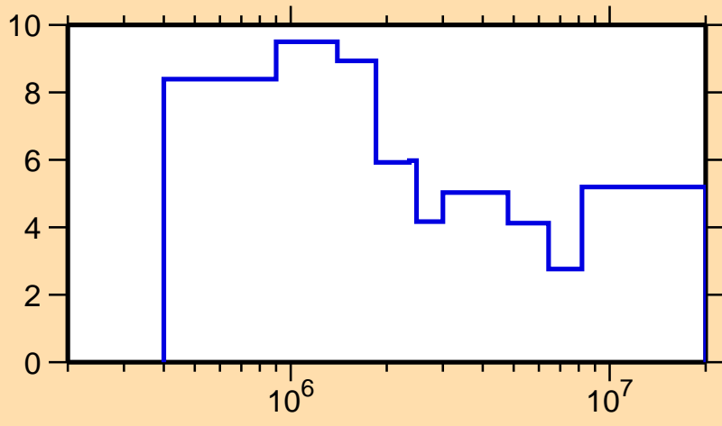
\Delta\sigma/\sigma vs. E for ^{76}\text{Br}(n,el.)
