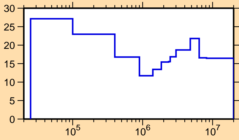
\Delta\sigma/\sigma vs. E for ^{76}\text{Br}(n,n_1)
